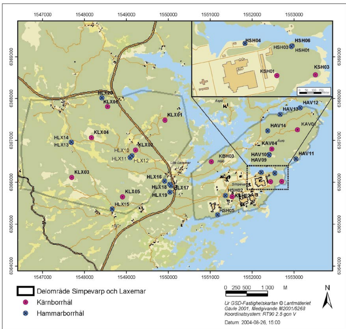
Figure 1-1. Location of the borehole KLX06A at the Oskarshamn site investigation area.
