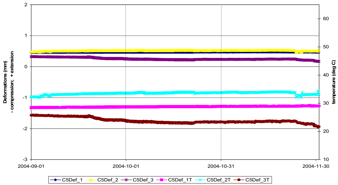
Vertical deformations adjacent to Deposition Hole 5 in borehole C5
