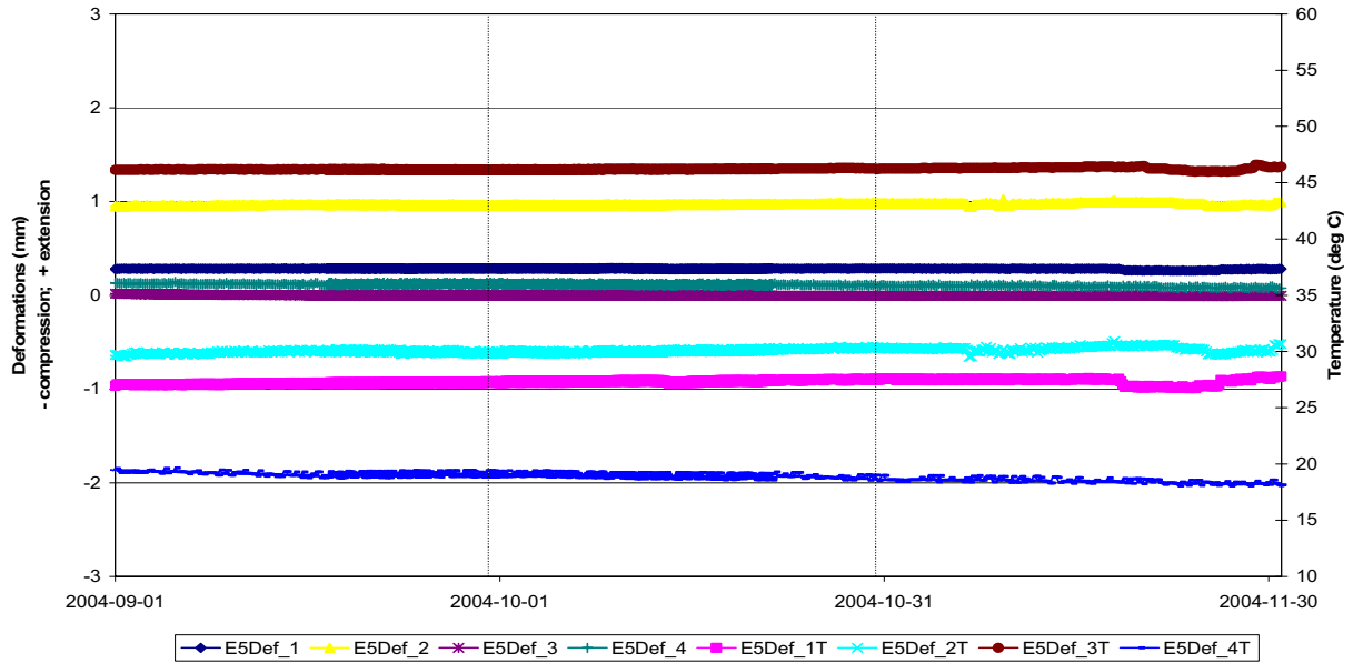
Vertical deformations adjacent to Deposition Hole 5 in Borehole E5
