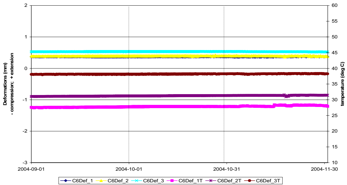
Vertical deformations adjacent to Deposition Hole 6 in borehole C6
