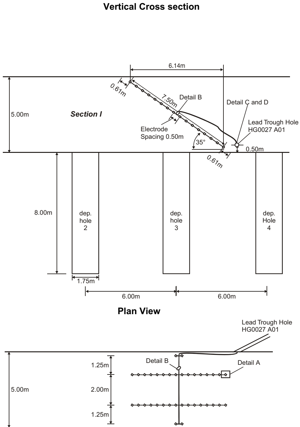
Figure 2-1: Electrode array in the backfill in section 1.
