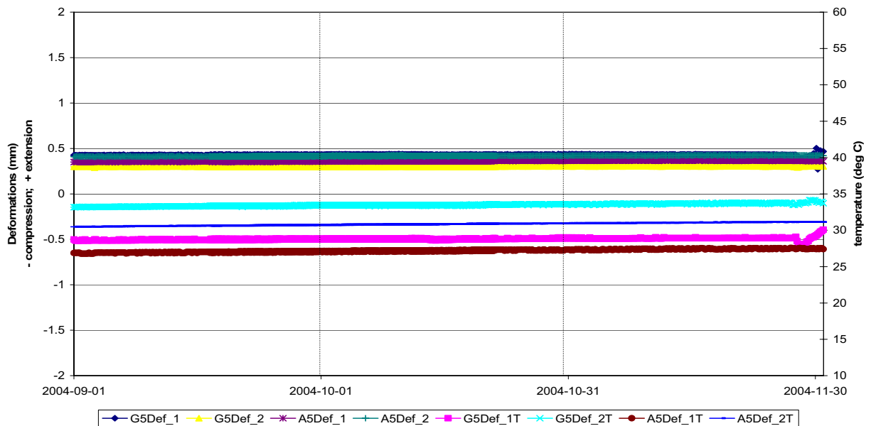
Vertical deformations adjacent to Deposition Hole 5 in Boreholes G5 and A5
