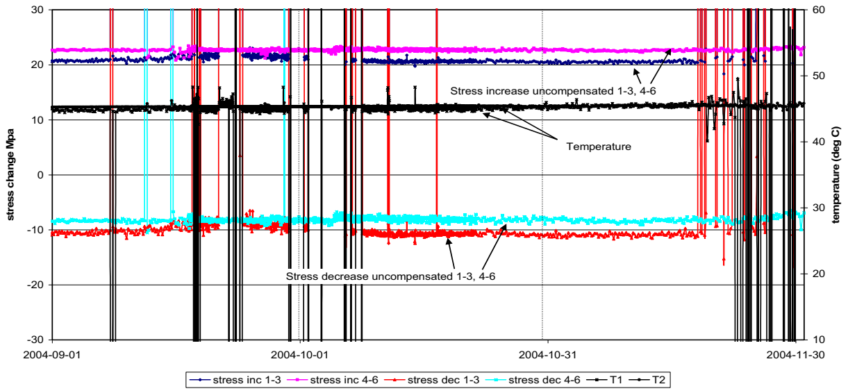
Biaxial stressmeter E5 Maximum stress increase and stress decrease in plane perpendicular to borehole axis
