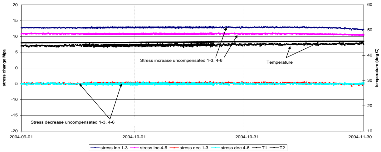
Biaxial stressmeter G5 Maximum stress increase and stress decrease in plane perpendicular to borehole axis
