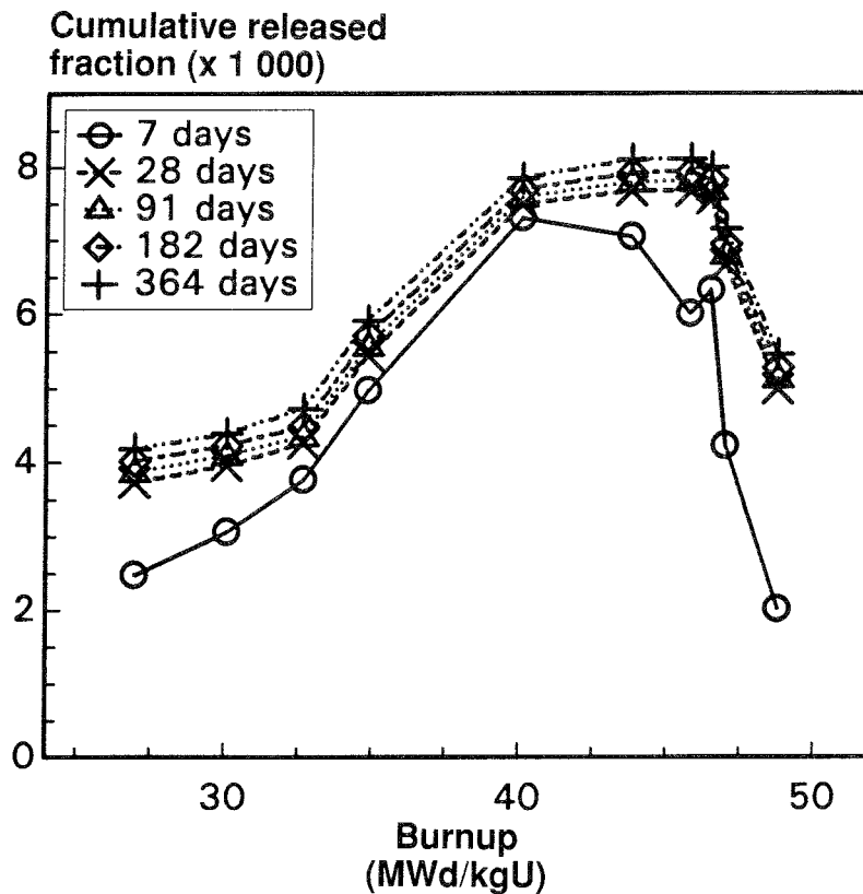
Figure 3-8. Cumulative released fraction of ^{137}\text{Cs} as a function of burnup (ground-water: oxidizing conditions).
