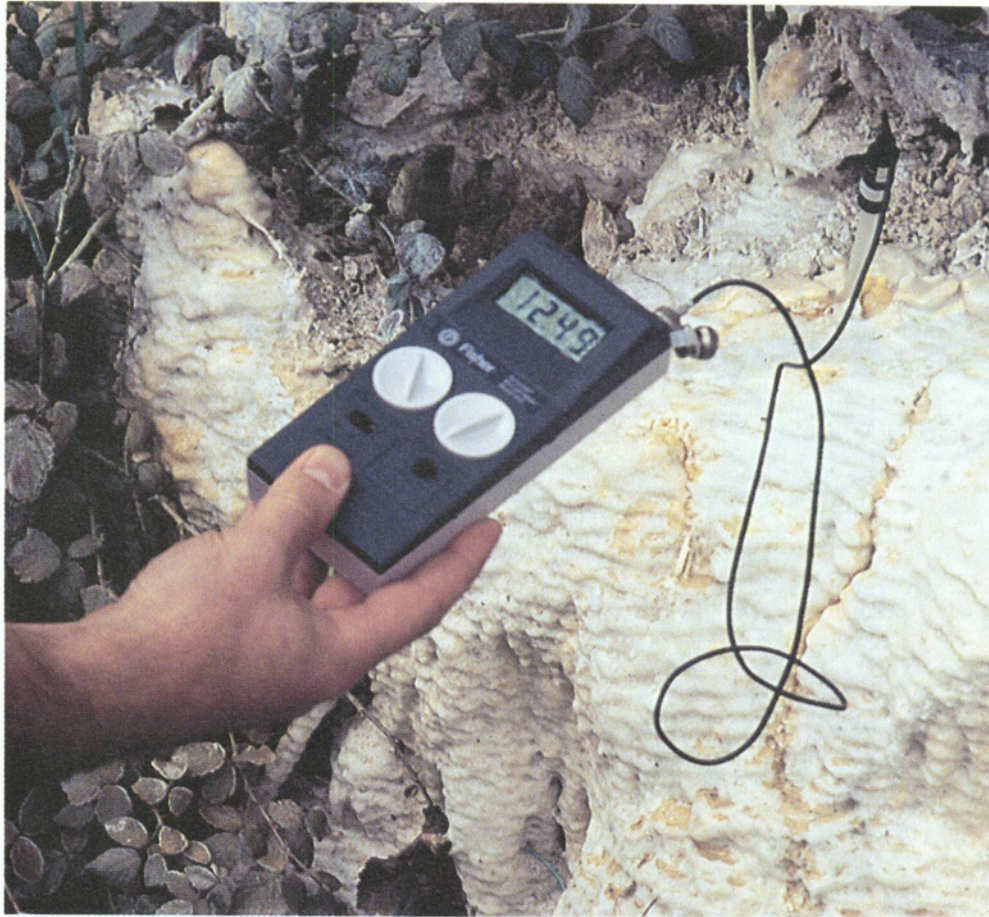
Figure 8-12. Measurement of pH in the hyperalkaline groundwater at Maqarin.
