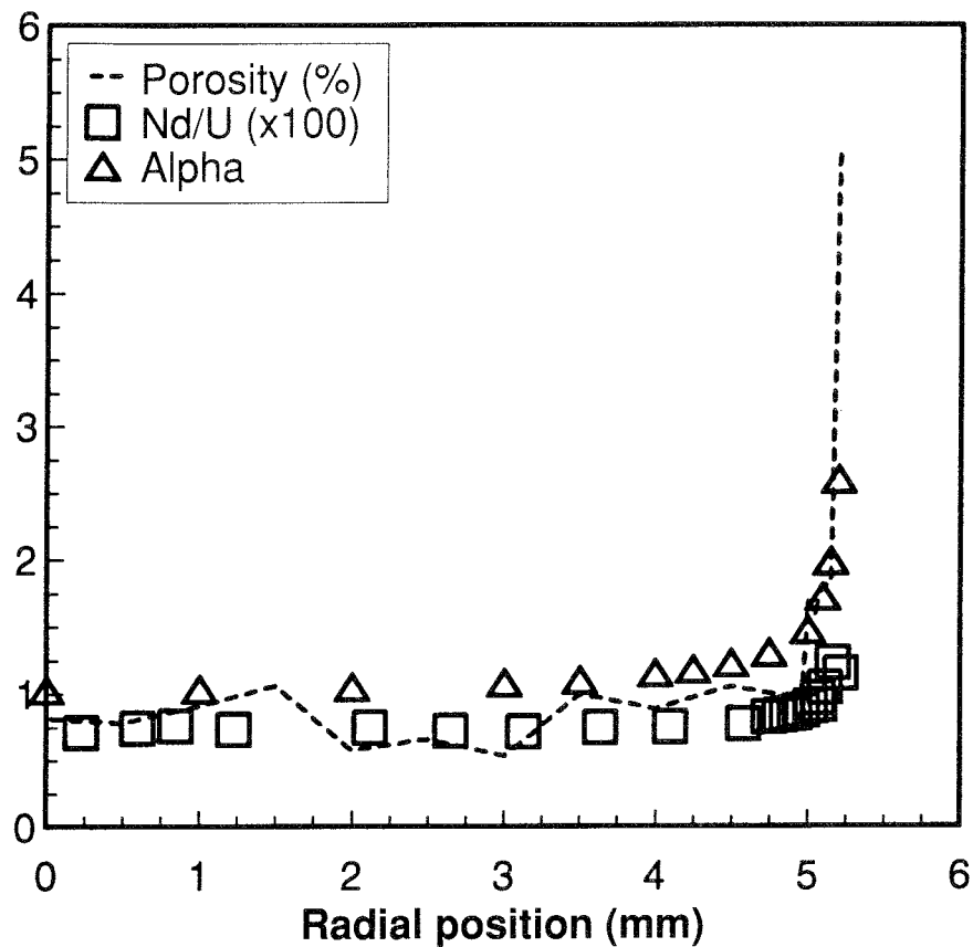
Figure 3-6. Radial variation of fuel porosity, burnup and alpha-activity in the reference fuel (BWR) from Oskarshamn-1.
