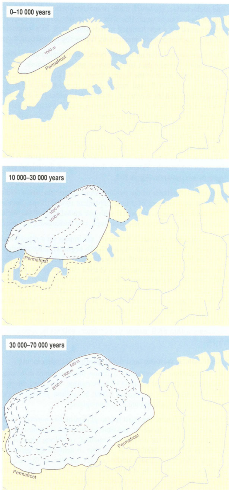
Figure 6-2. Extent of future inland ice sheets according to SKB/TVO's ice age scenario.
