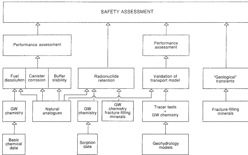
Figure 7-5. Illustration of how different kinds of data are used to model and validate transport.
