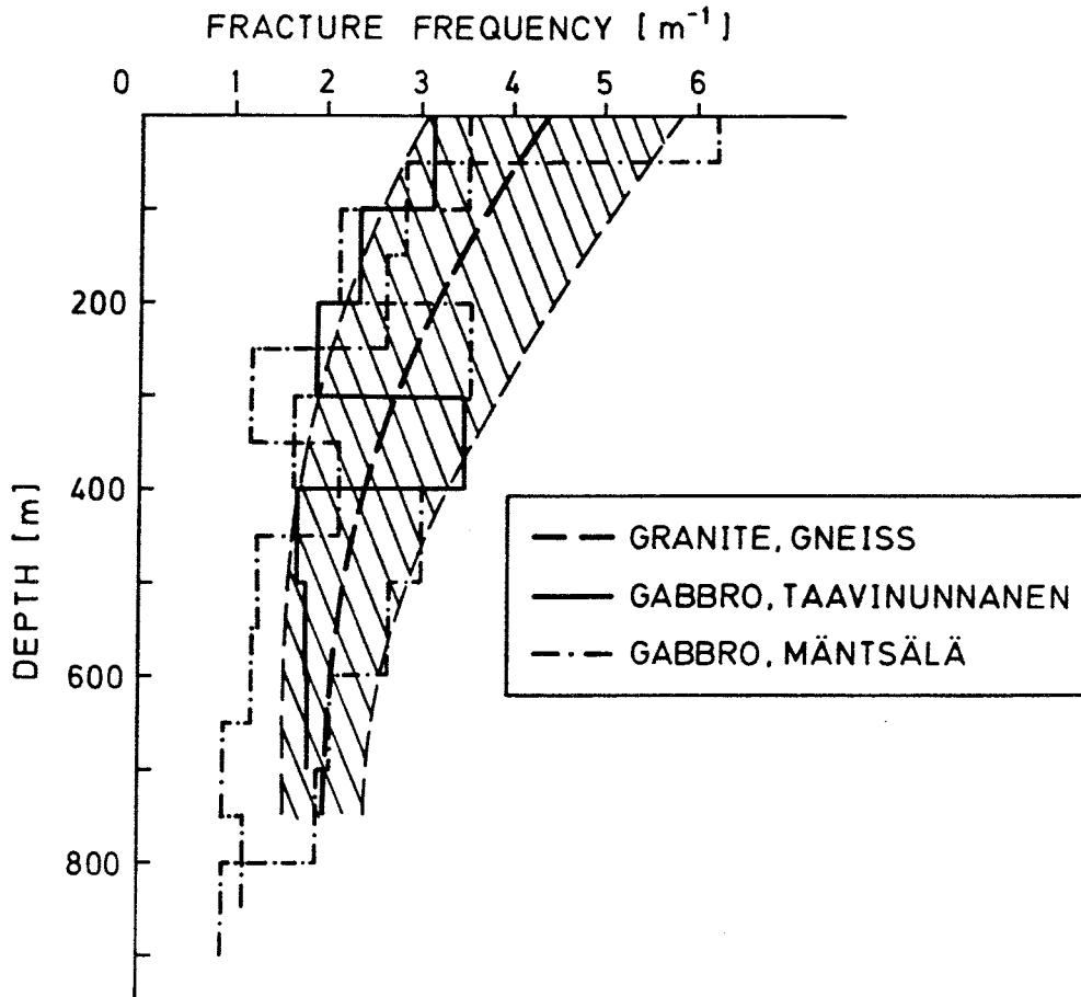
Figure 12. Fracture frequency as a function of depth. Histograms show data obtained from gabbro intrusions (Taavinunnenen and Mäntsälä). Shaded area shows average and approximate range of variation for granitic rocks at Swedish study sites.
