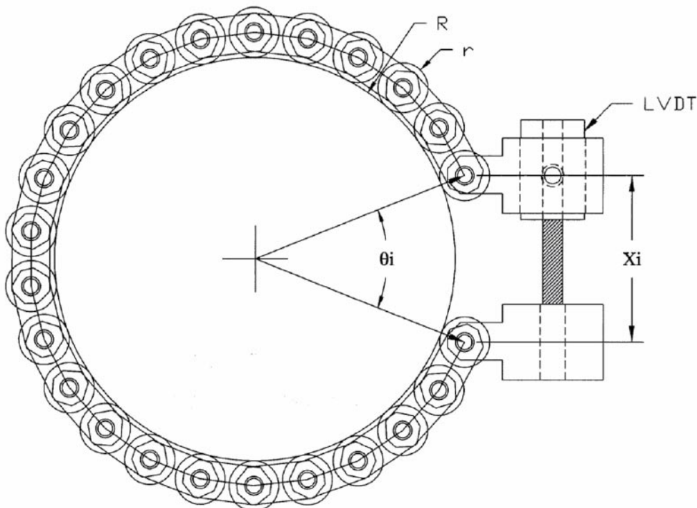
Figure A-1. Chain for radial deformation measurement.
