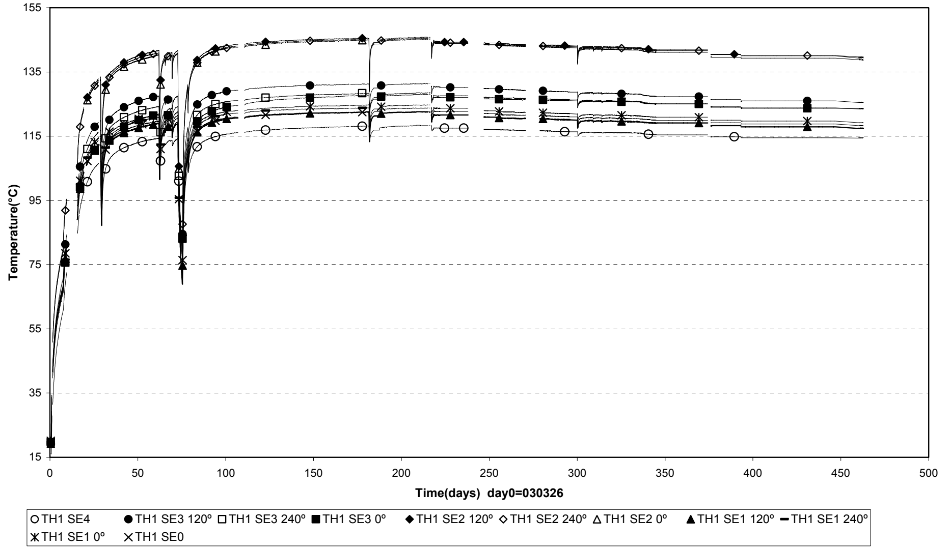
External temperatures Heater 1 (030326-040701)
