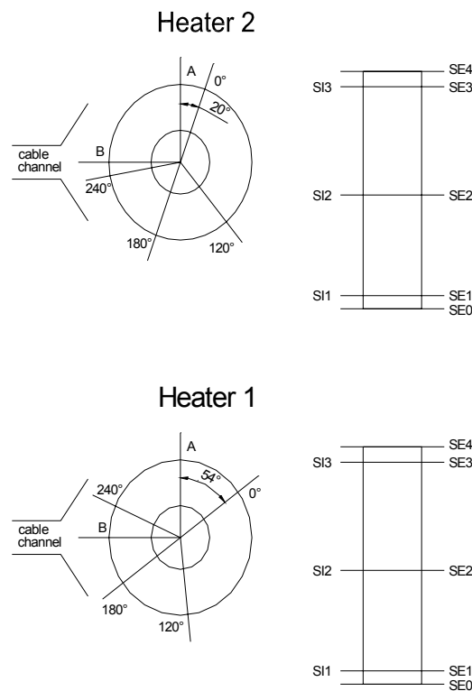
Figure 4-2. Location of thermocouples inside (SI) and on (SE) the canisters
