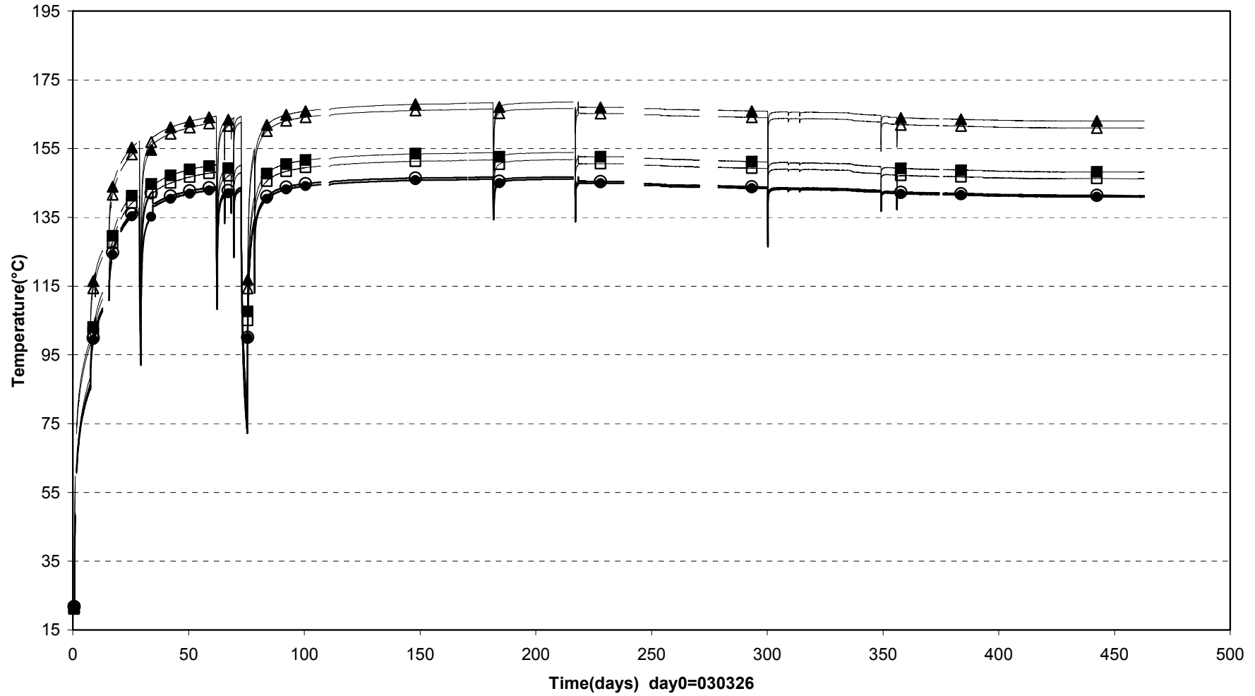
Internal temperatures Heater 1 (030326-040701)
