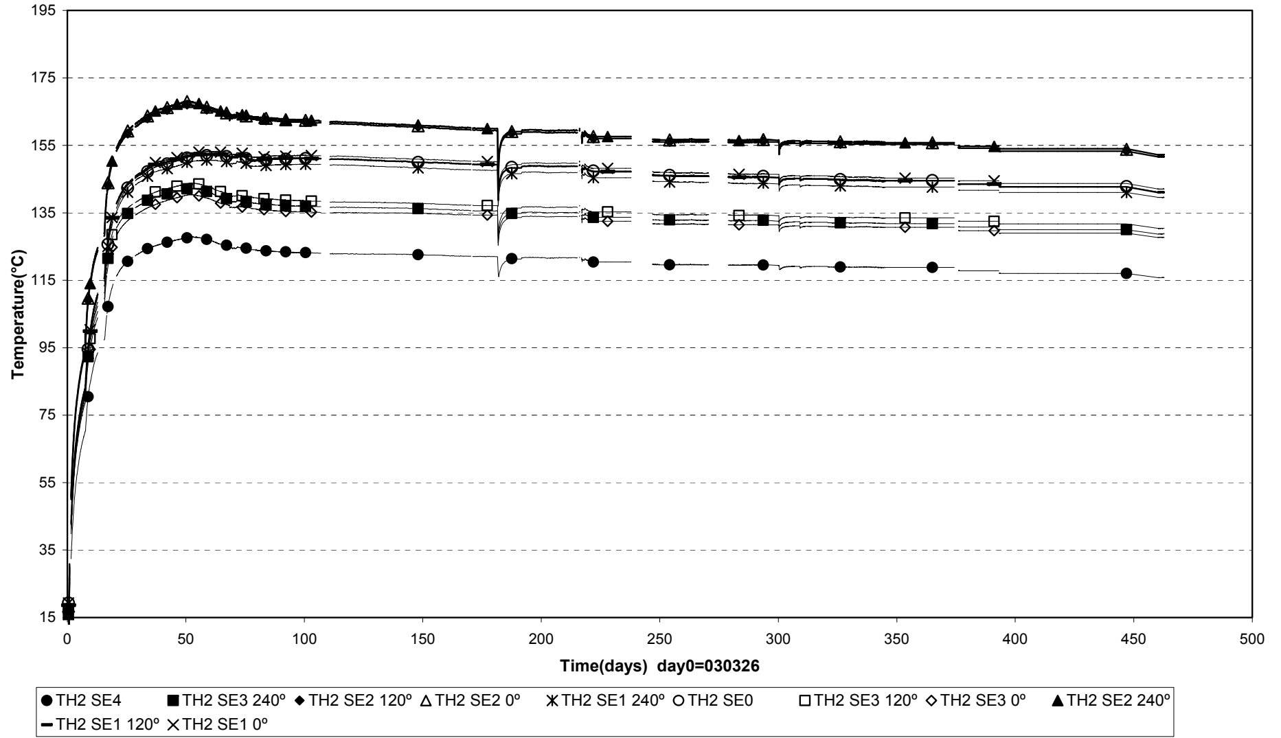
External temperatures Heater 2 (030326-040701)
