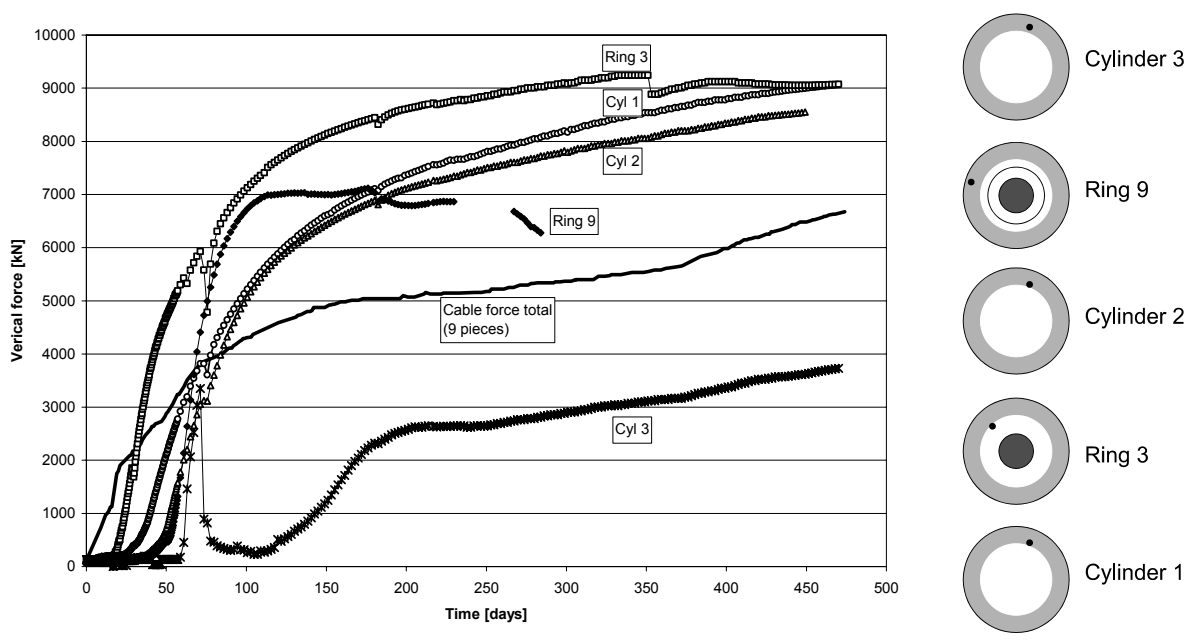
Figure 5-5. Axial pressure measurement translated into vertical forces, assuming annular region shown to the right (grey-shaded) to be involved in force transfer. The black dots show the stress measurement positions.
