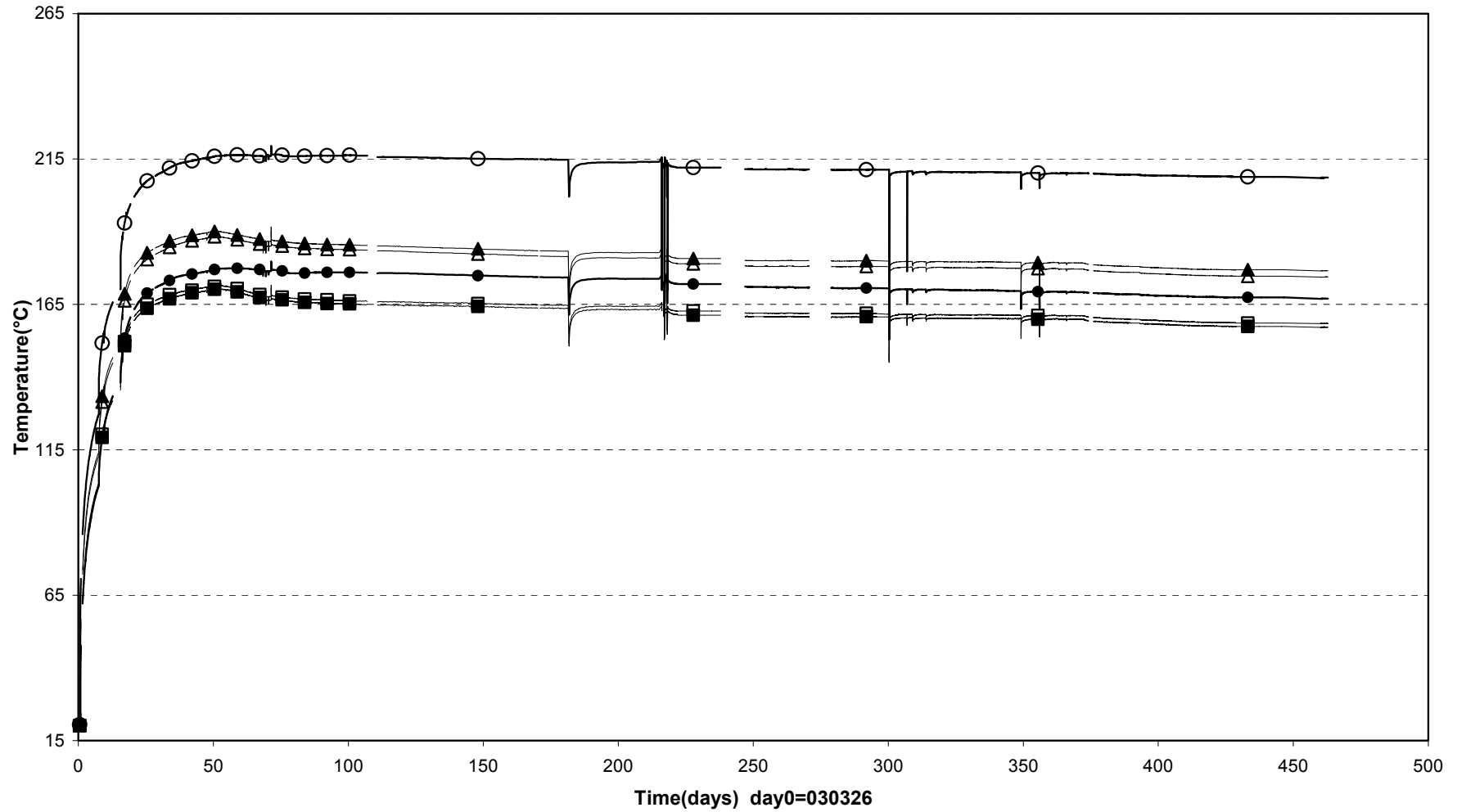
Internal temperatures Heater 2 (030326-040701)
