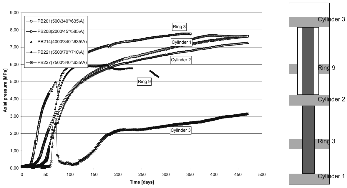
Figure 5-4. Axial pressure measured in different sections. Sensor in Ring 9 failed after about 300 days.
