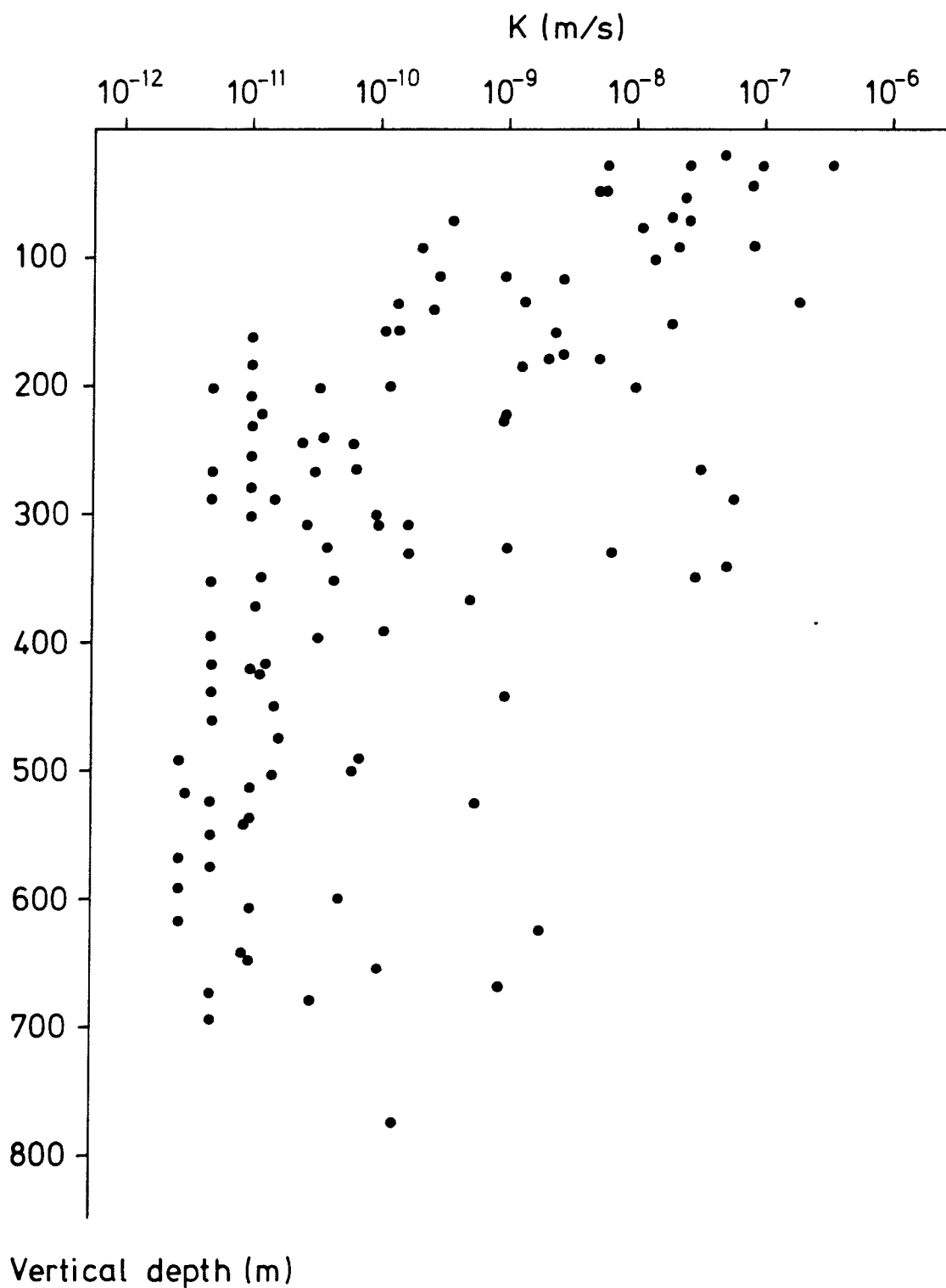
Figure 7.4 Hydraulic conductivity for the rock mass in the drill holes Sv 1, Sv 3-Sv 7 (25 m sections).
