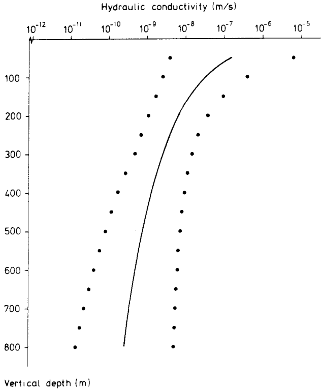
Figure 7.7. Relationship between hydraulic conductivity and depth in local fracture zones.
