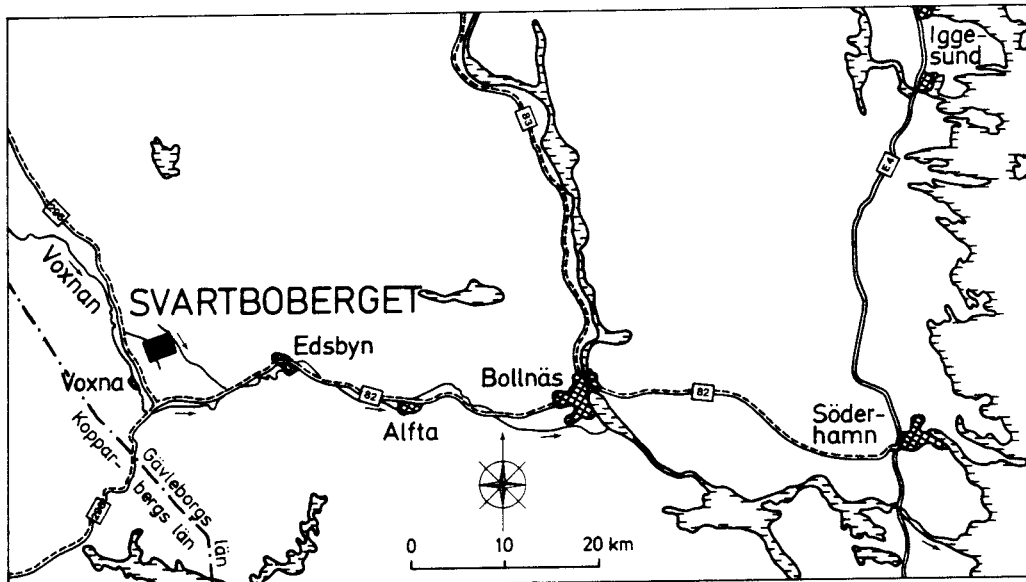
Figure 3.1. Locality map of site Svartboberget.
