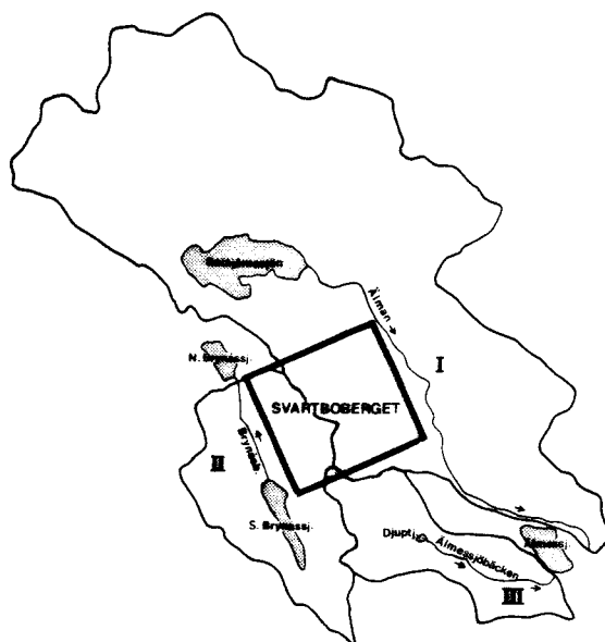
Figure 6.1. Local drainage areas within site Svartboberget.
