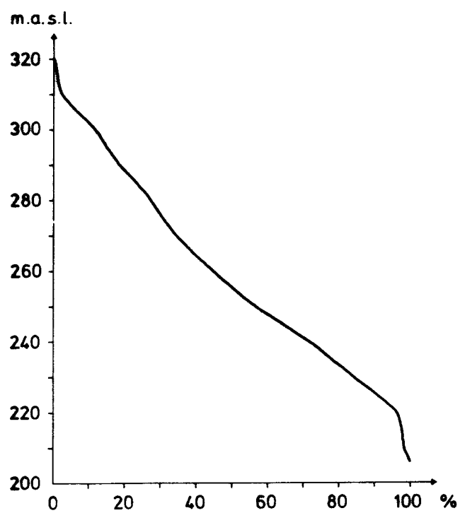
Figure 3.3. Hypsographical curve showing altitude characteristics in site Svartboberget.
