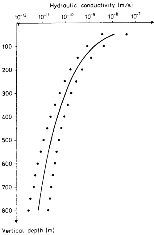
Figure 7.6. Relationship between hydraulic conductivity and depth in the rock mass.
