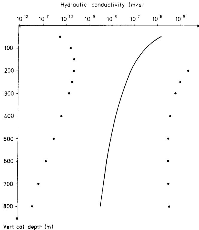
Figure 7.8. Relationship between hydraulic conductivity and depth in regional fracture zones.
