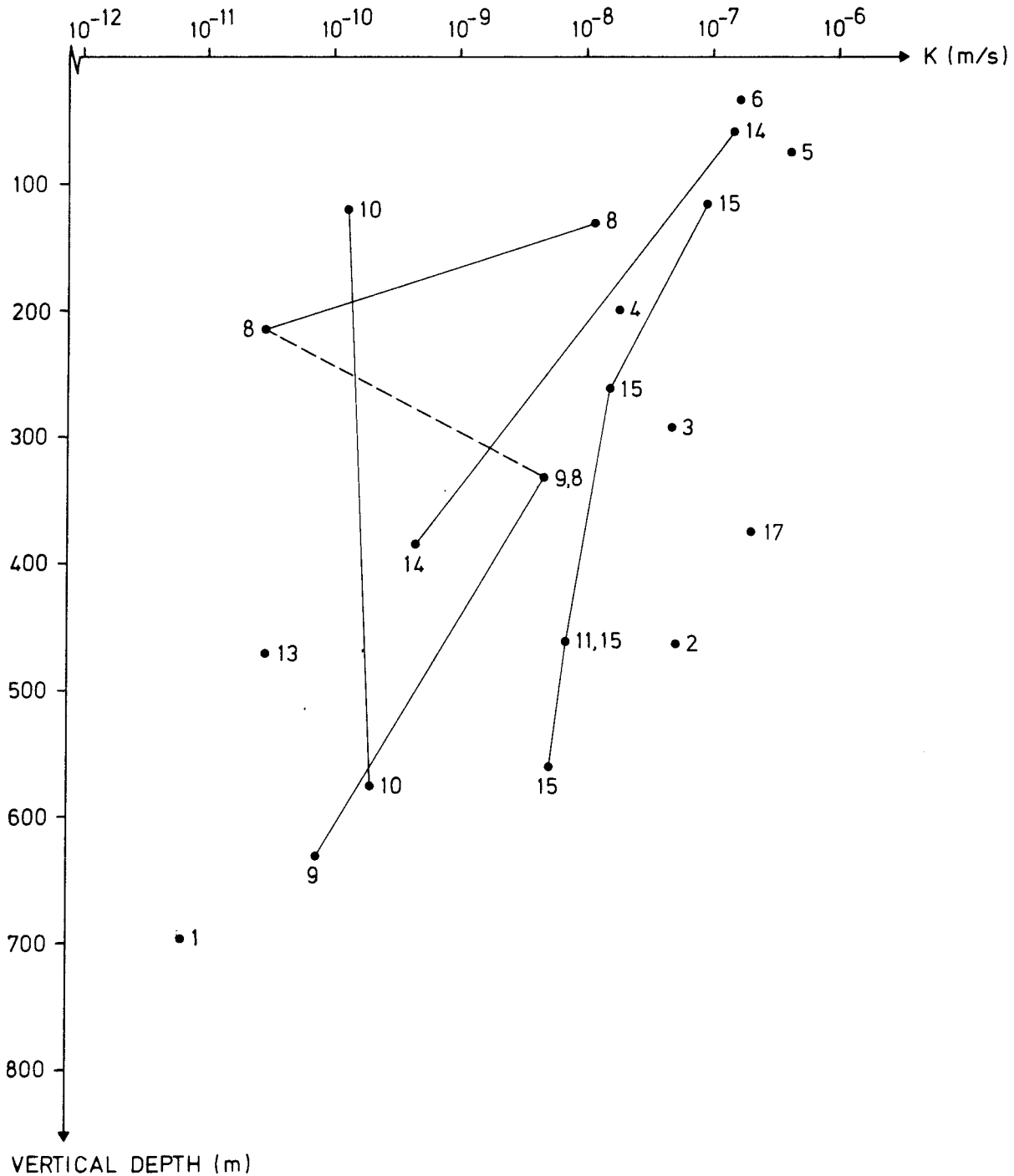
Figure 7.5. Hydraulic conductivity in local fracture zones penetrated by the drill holes Sv 1, Sv 3-Sv 7.
