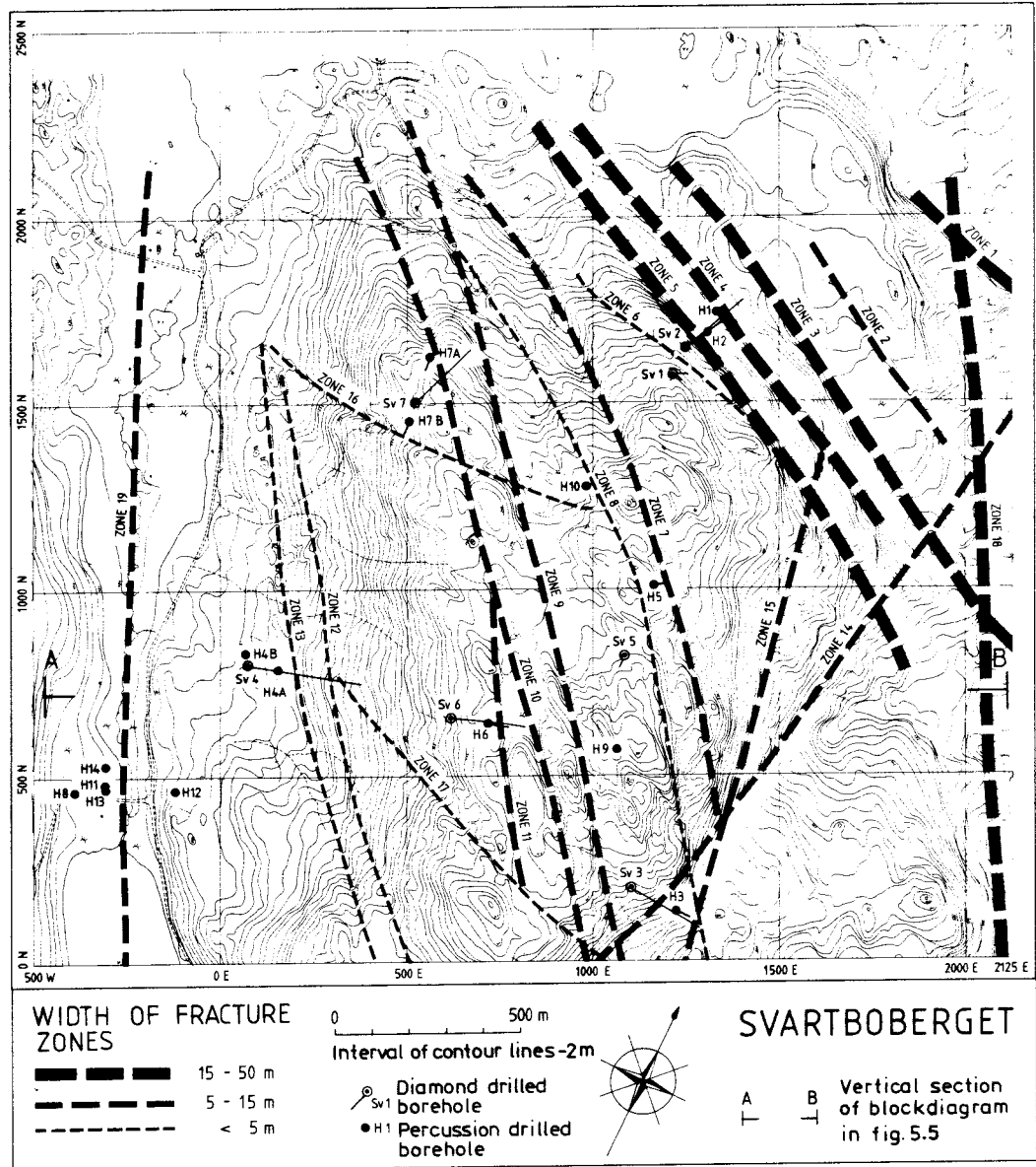
Figure 5.4 Fracture zones at the surface of site Svartboberget.
