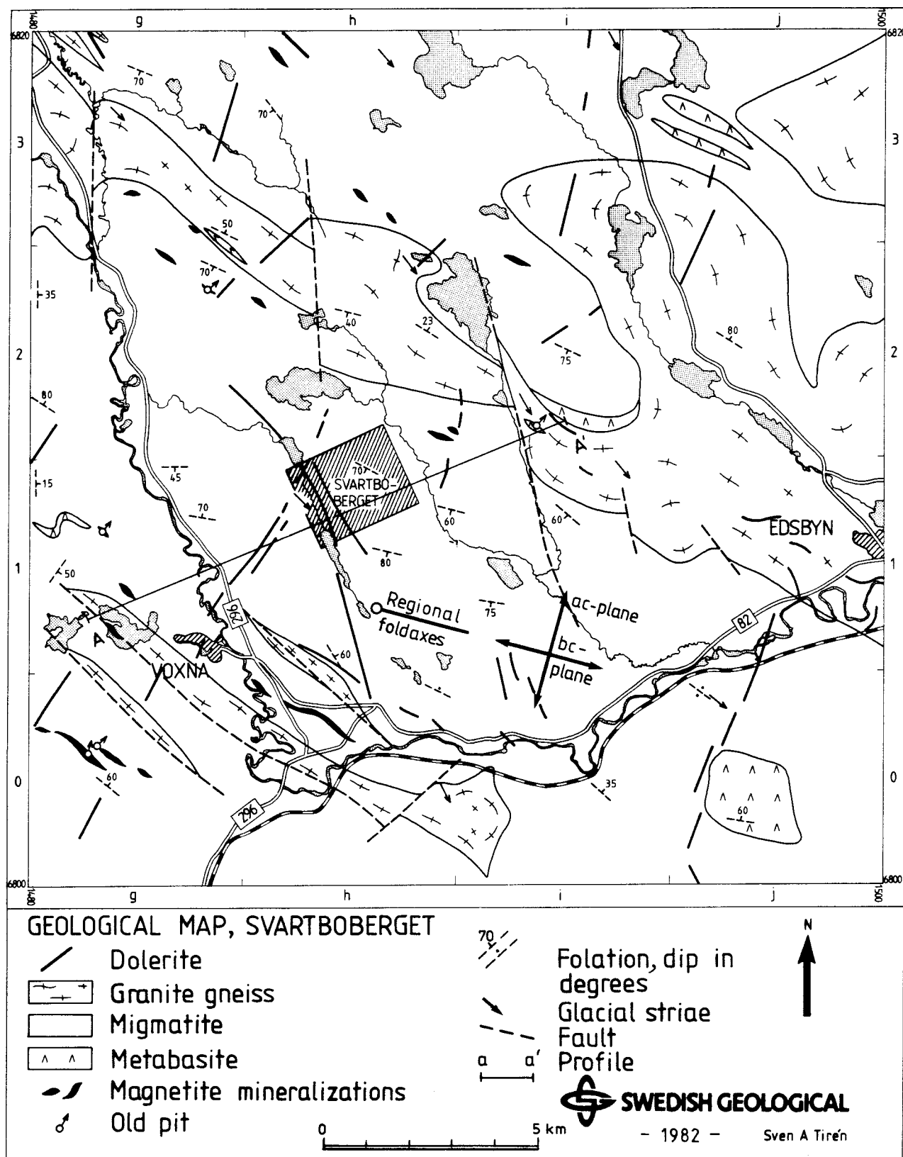
Figure 4.1. Regional geological map including site Svartboberget.
