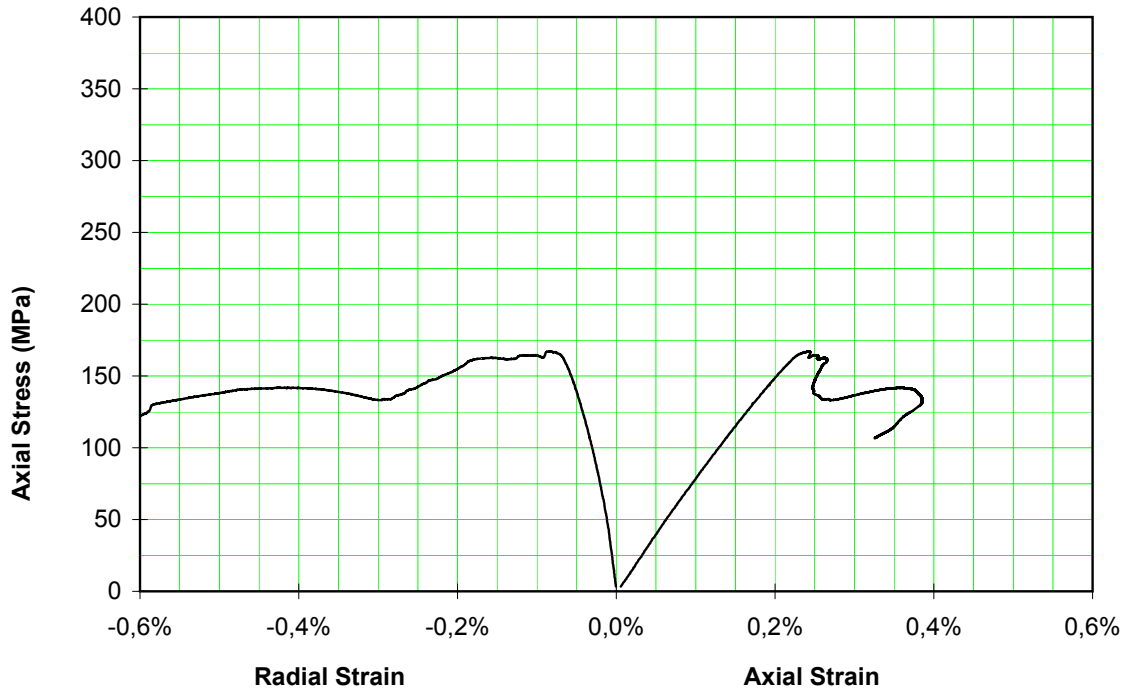
STRESS - STRAIN CURVES
