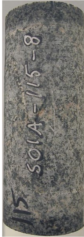
(b) After testing (2004-05-10)
