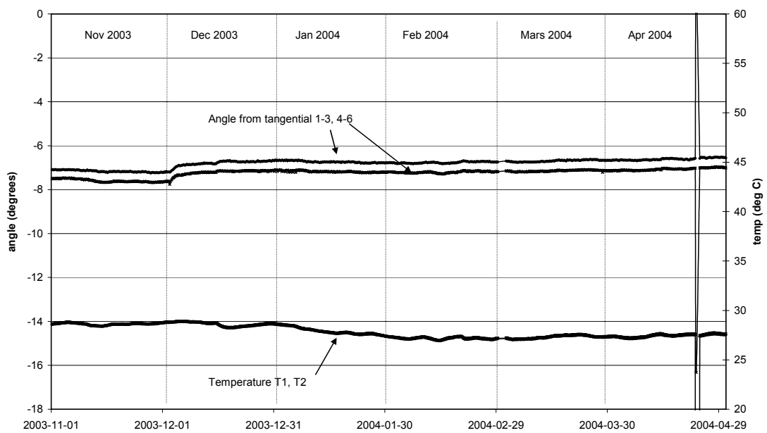
Biaxial stressmeter A2 Orientation of maximum stress increase in plane perpendicular to borehole axis
