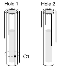
Biaxial stressmeter C1 Maximum stress increase and stress reduction in plane perpendicular to borehole axis
