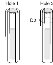
Biaxial stressmeter D2 Maximum stress increase and stress reduction in plane perpendicular to borehole axis
