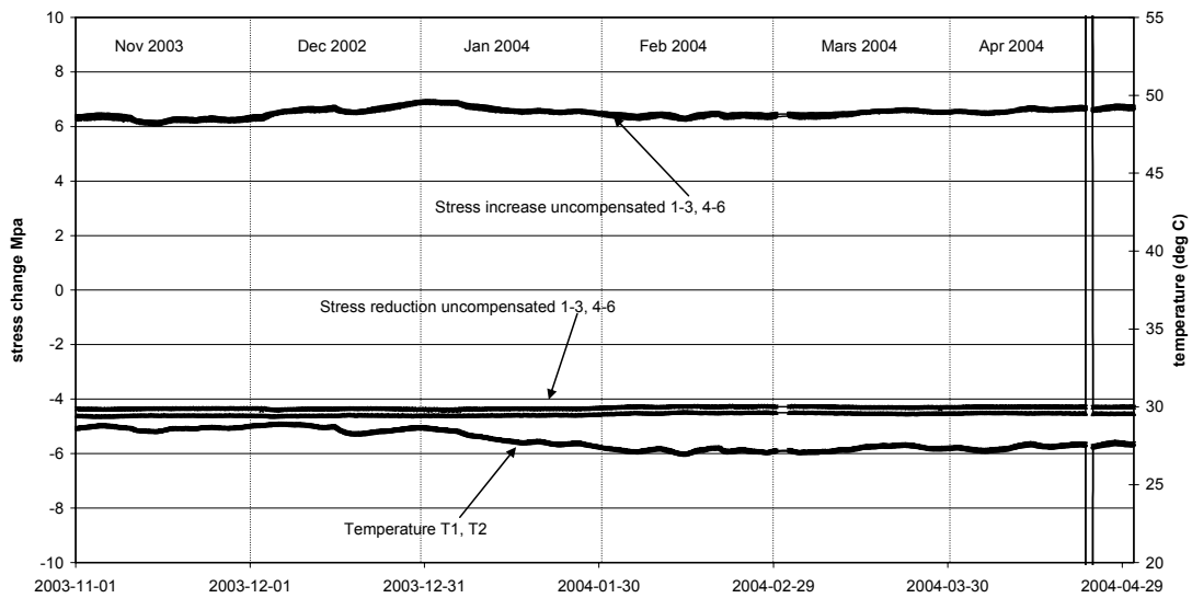
Biaxial stressmeter A2 Maximum stress increase and stress decrease in plane perpendicular to borehole axis
