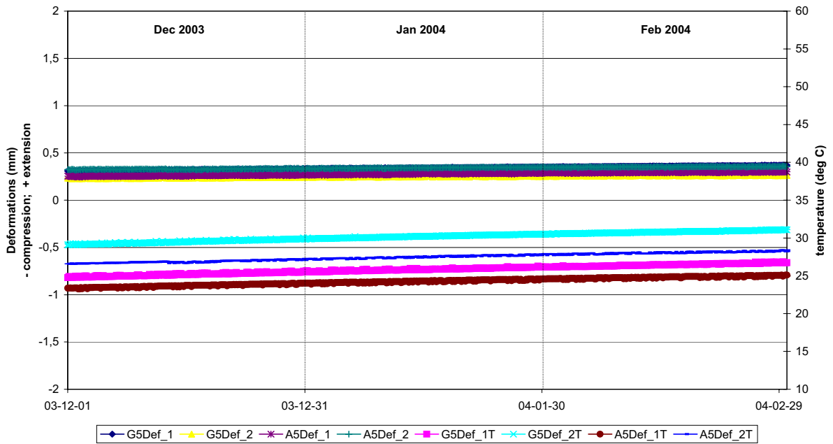
Vertical deformations adjacent to Deposition Hole 5 in Boreholes G5 and A5
