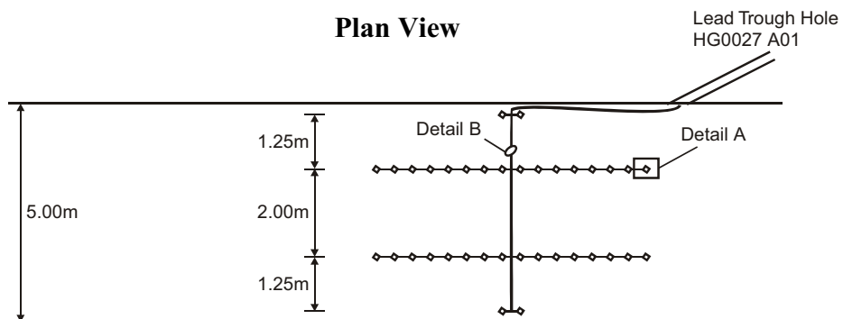
Figure 2-1: Electrode array in the backfill in section 1.
