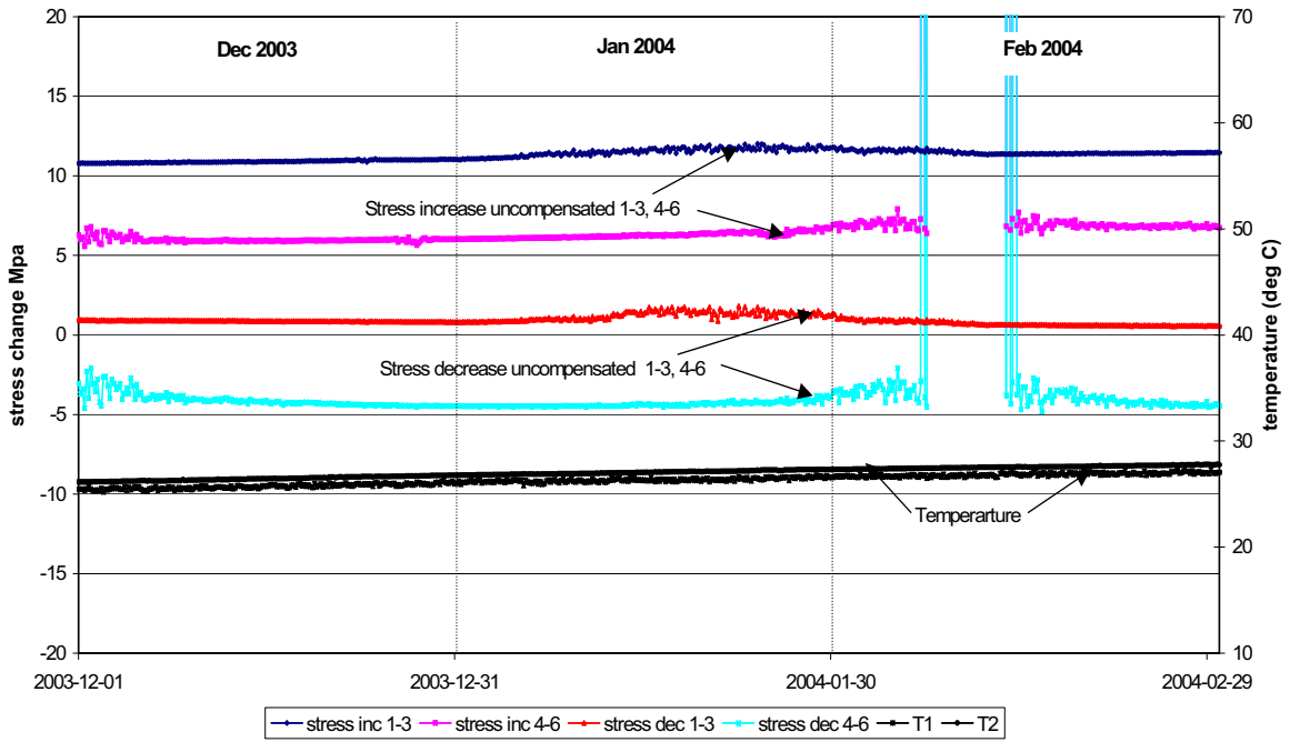
Biaxial stressmeter A6 Maximum stress increase and stress decrease in plane perpendicular to borehole axis
