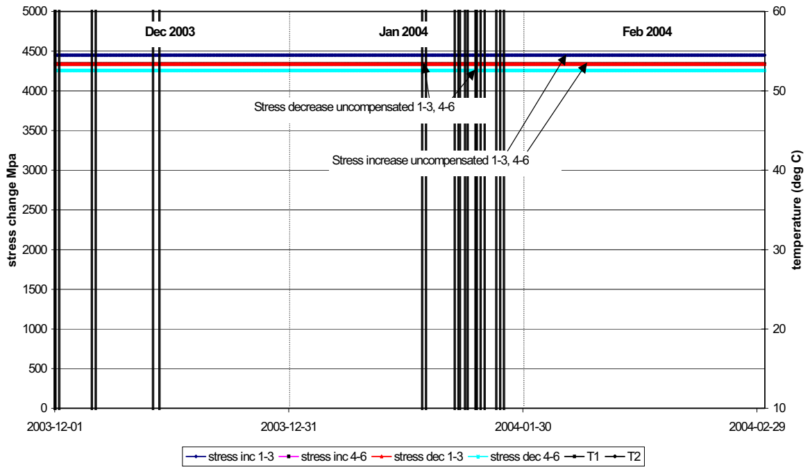
Biaxial stressmeter C6 Maximum stress increase and stress decrease in plane perpendicular to borehole axis
