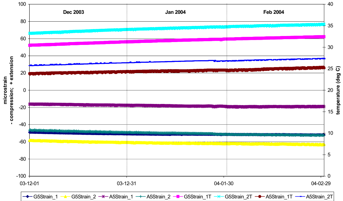
Vertical strain adjacent to Deposition Hole 5
