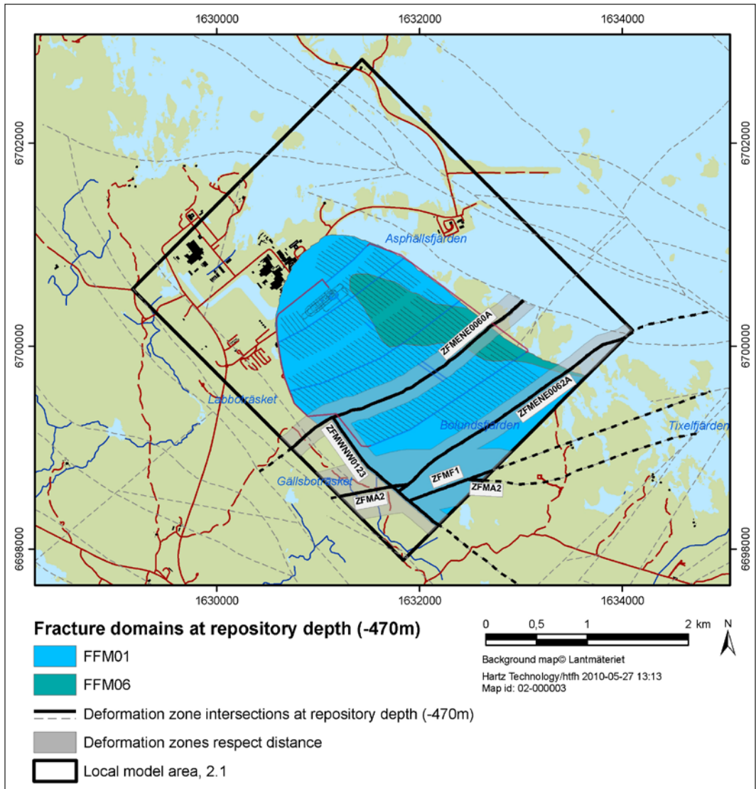
Figure 4-1. Deformation zones with respect distances which impact the repository layout. Section at repository depth (-470 m) 1 .
