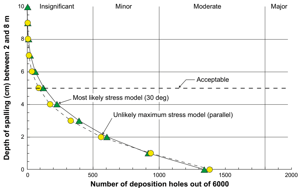
Figure 4-3. Loss of deposition holes for the “Most likely” stress model with the deposition tunnels at 30 degrees to the maximum horizontal stress and the “Unlikely maximum” stress model with the deposition tunnel parallel to the maximum horizontal stress /SKB 2009b/.
