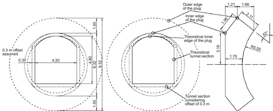
Figure 2-3. Nominal geometry for the plug.
