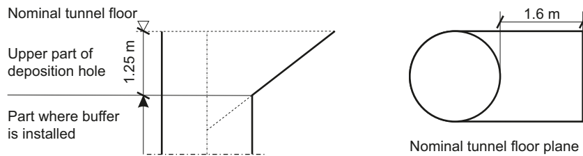
Figure 5-2. The nominal dimensions of the bevel. This upper part of the deposition hole is regarded as part of the deposition tunnel.
