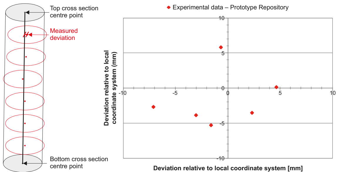
Figure B-1. Deviation was defined as the horizontal distance between the theoretical centre point of the cross-section in question and a reference line between the theoretical centre point at the bottom of the hole and the theoretical centre point at the top. This measure can be regarded as an estimation of the straightness of the deposition hole. Calculation results showing the maximum deviation value are plotted for each deposition hole.
