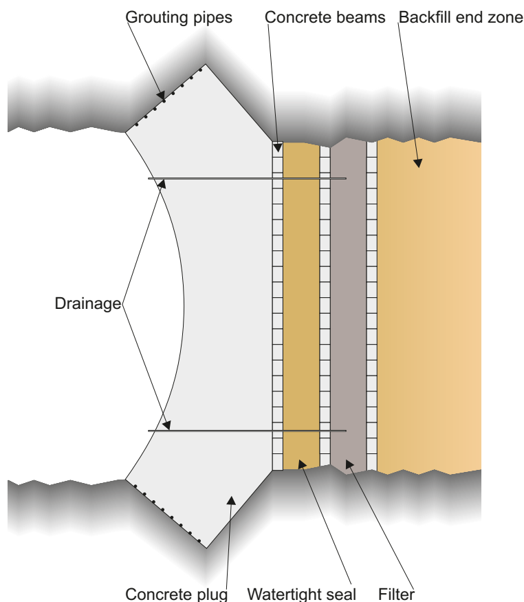
Figure 5-1. Schematic illustration of a reinforced plug that is anchored in a recess in the rock around the deposition tunnel.
