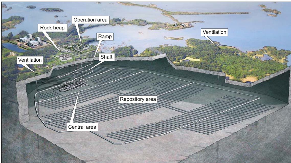
Figure 3-1. Illustration of the layout contained in the D2 Reference Design for a final repository facility in Forsmark.
