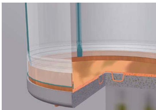
Figure 5-3. The bottom plate in the deposition hole.
