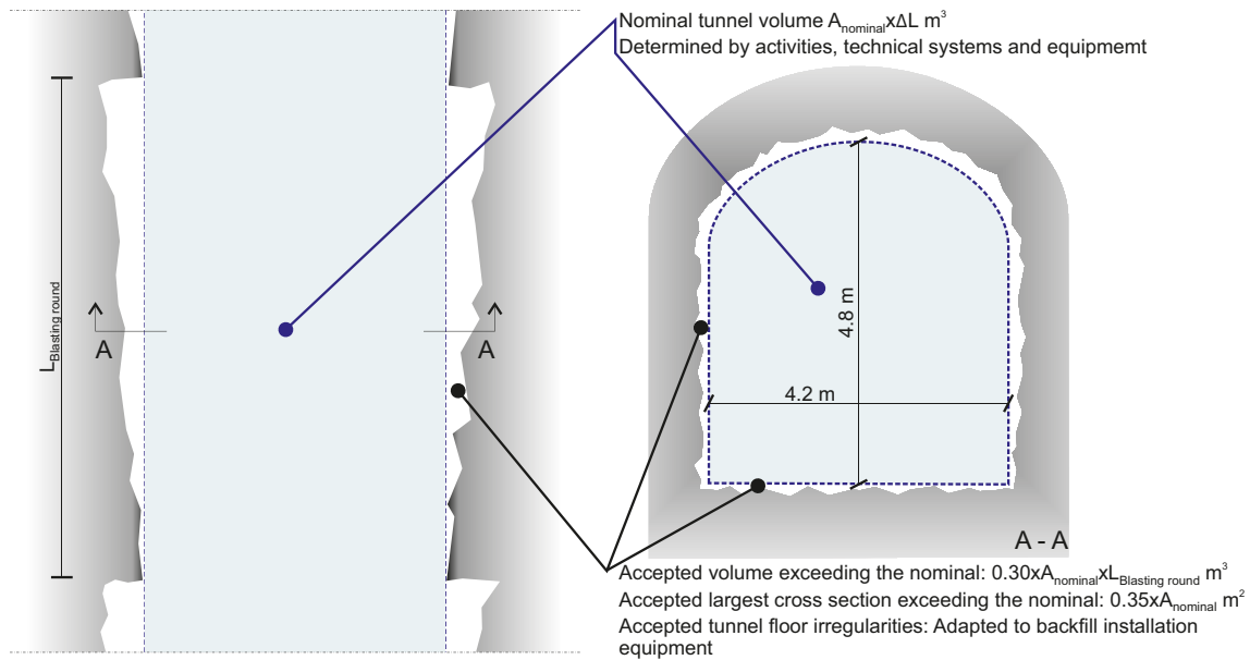
Figure 2-2. Nominal tunnel geometry and acceptable volume of rock fall out and irregularities in the tunnel walls.
