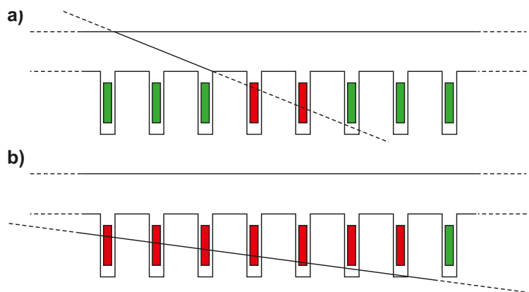
Figure 4-2. Illustration of a) the FPC criterion (Full Perimeter Intersection criterion) and b) the EFPC criterion (Extended Full Perimeter Intersection criterion). Red positions are rejected, green positions are accepted.
