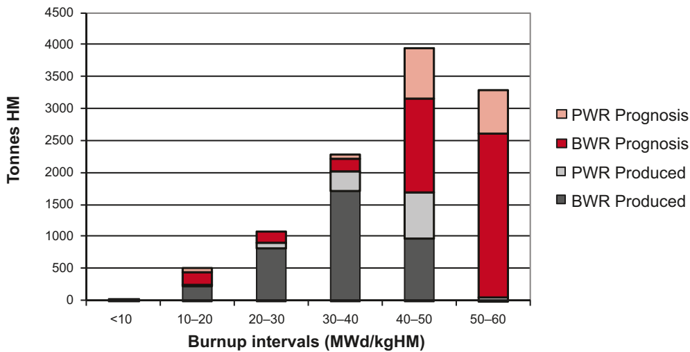
Figure 2-2. Average burnup distribution per tonne heavy metal of the BWR and PWR fuel stored in Clab 31 December 2007 (grey colours) and prognosis of the burnup distribution for the future operation of the nuclear power plants (red colours) as assumed for the reference scenario used by SKB.
