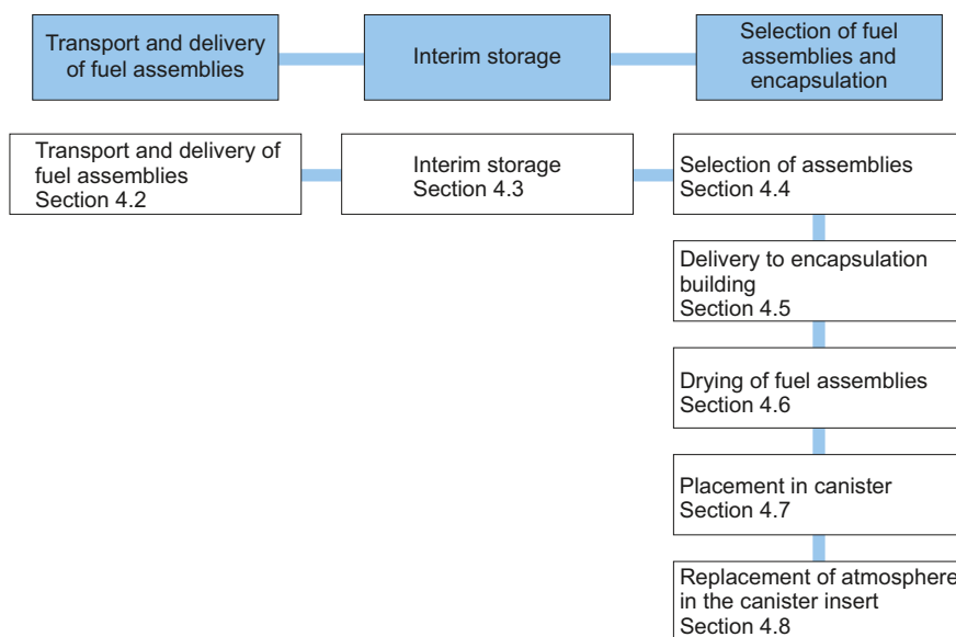
Figure 4-1. Flow chart for the spent fuel line and its stages. A flow chart for the handling of the encapsulated spent fuel is provided in the Canister production report, Figure 6-1.
