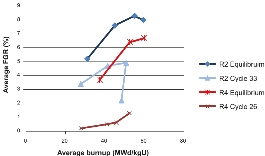
Figure 6-3. Calculated average fission gas release at the end of each cycle for the PWR cases. The drop in burnup and FGR for R2 (Ringhals 2) Cycle 33 is explained by that only the low burnup assemblies were loaded in the last cycle.
