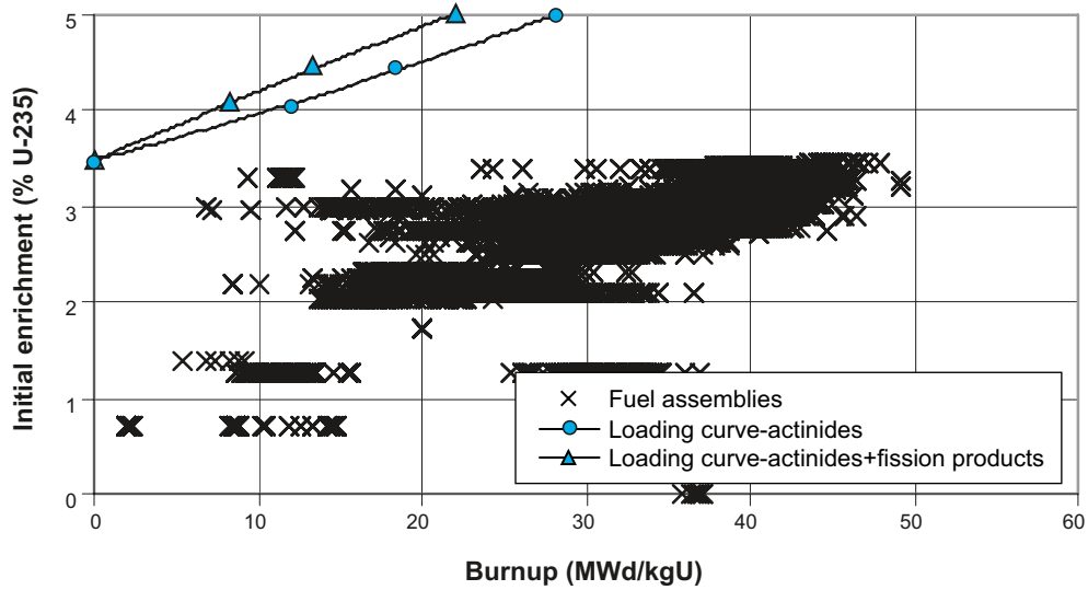
Figure 4-3. Loading curves for BWR-canisters with 12 identical fuel assemblies and enrichment and average burnup for the assemblies currently stored in Clab /SKBdoc 1193244/.
