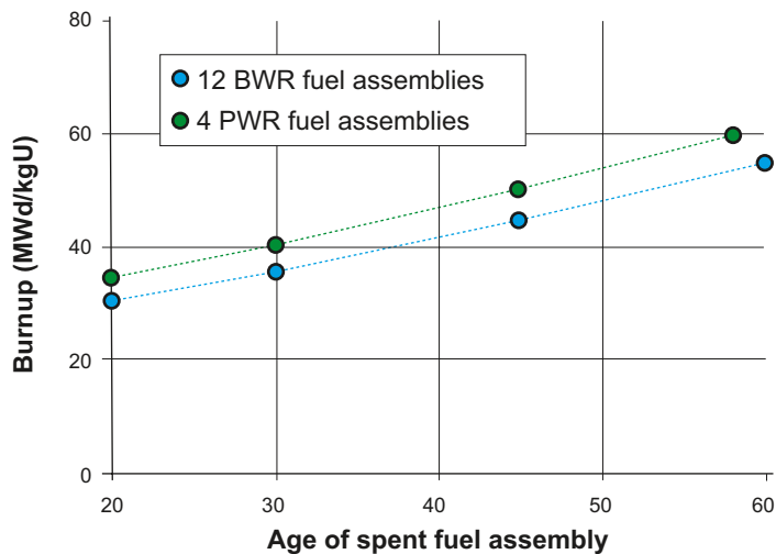
Figure 5-1. Burnup and age of spent fuel assembly required to reach a decay power of 1,700 W in a BWR and PWR canister respectively assuming that all positions are occupied by assemblies with the same decay power:
