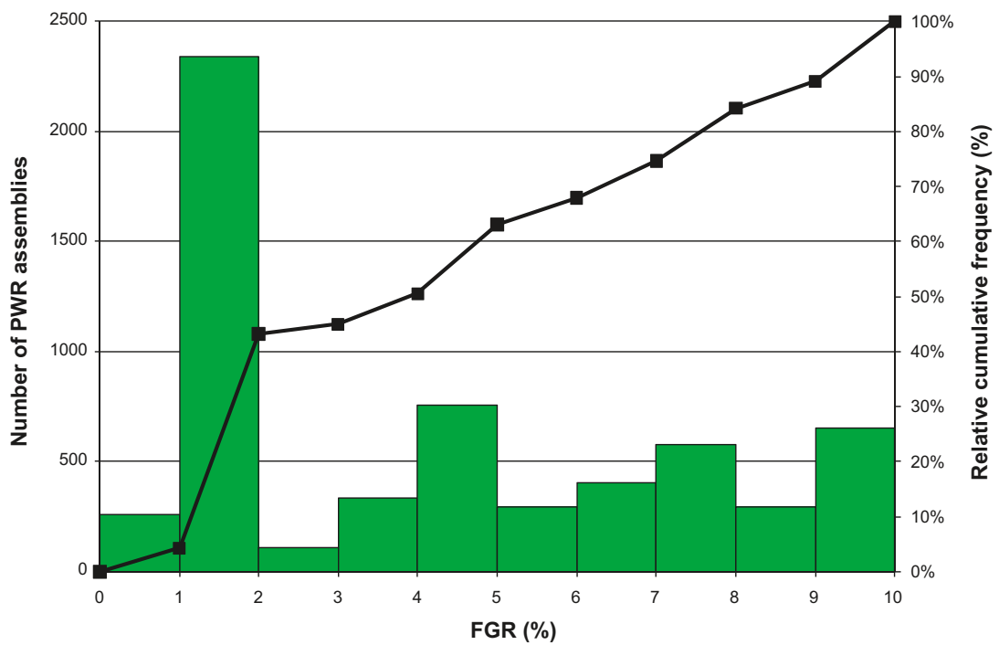
Figure 6-5. The number of PWR assemblies in different FGR intervals and relative cumulative frequency of FGR in PWR assemblies.
