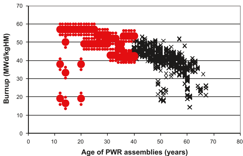
Figure 2-4. The burnup and age in 2045 of the PWR assemblies included in the reference scenario. Assemblies that are currently stored in Clab are marked with black and assemblies from the future operation are marked with red. Large red dots represent batch average discharge burnup and small red dots represent standard deviation in burnup, i.e. \pm 3 MWd/kgU, averaged over single fuel assemblies included in a batch.
