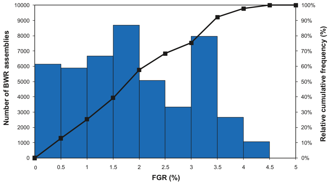
Figure 6-4. The number of BWR assemblies in different FGR intervals and relative cumulative frequency of FGR in BWR assemblies.
