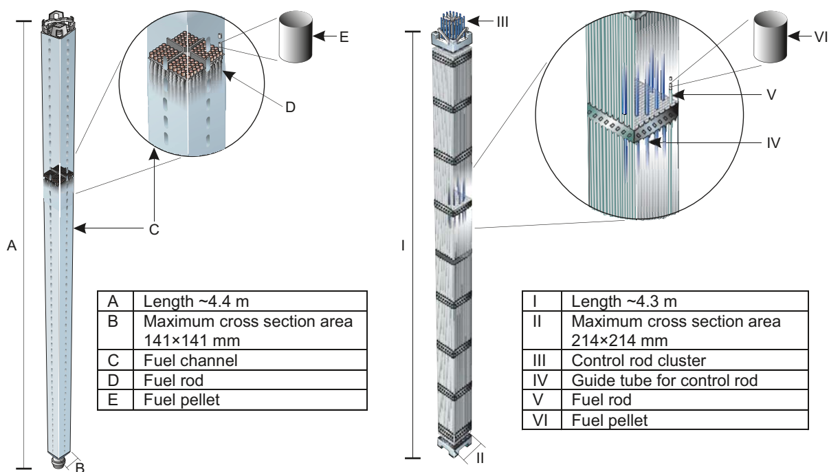
Figure 2-5. Arbitrary BWR (left) and PWR (right) assemblies. Data based on specifications provided by the nuclear fuel suppliers.
