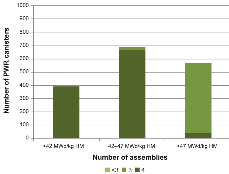
Figure 5-3. The PWR canisters to be deposited divided into groups with respect to the average burnup of the encapsulated assemblies. The number of assemblies in the canister is indicated by different colours. The total number of PWR canisters is 1,652.
