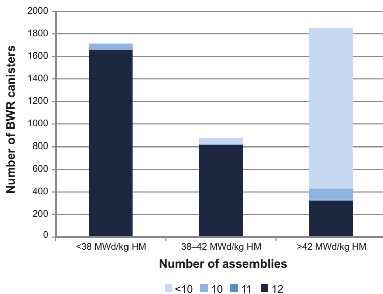
Figure 5-2. The BWR canisters to be deposited divided into groups with respect to the average burnup of the encapsulated assemblies. The number of assemblies in the canister is indicated by different colours. The total number of BWR canisters is 4,451.
