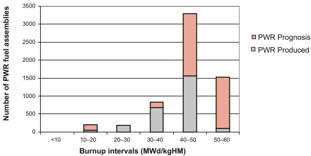
Figure 2-1. Burnup distribution of the spent fuel assemblies stored in Clab 31 December 2007 (grey colours) and prognosis of the burnup distribution for the assemblies resulting from the future operation of the nuclear power plants (red colours) as assumed for the reference scenario used by SKB.
