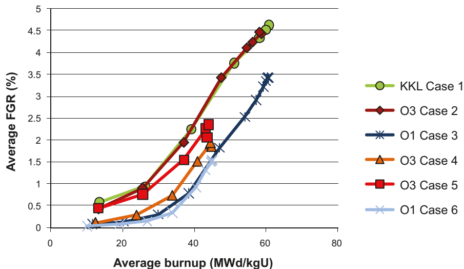
Figure 6-2. Calculated average fission gas release at the end of each cycle for the BWR cases.
