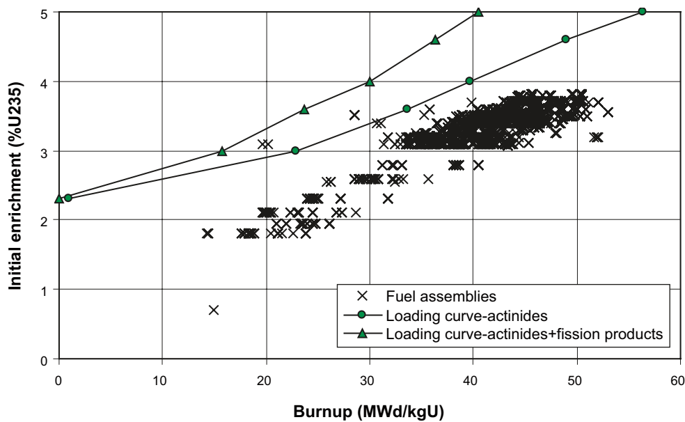
Figure 4-4. Loading curves for PWR-canisters with 4 identical fuel assemblies and enrichment and average burnup for the assemblies currently stored in Clab /SKBdoc 1193244/.
