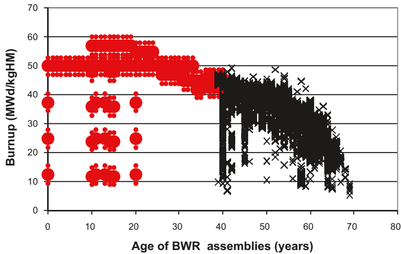
Figure 2-3. The burnup and age in 2045 of the BWR assemblies included in the SKB reference scenario. Assemblies that are currently stored in Clab are marked with black and assemblies from the future operation are marked with red. Large red dots represent batch average discharge burnup and small red dots represent standard deviation in burnup, i.e. \pm 3 MWd/kgU, averaged over single fuel assemblies included in a batch.
