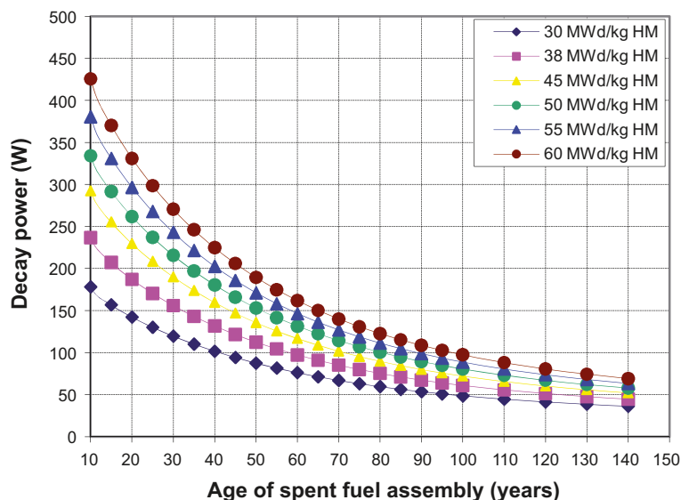
Figure 4-2. The decay power as a function of age for BWR assemblies with different burnup. (The allowed average decay power per encapsulated assembly is 142 W for a canister with 12 identical assemblies.) /SKBdoc 1198314/.
