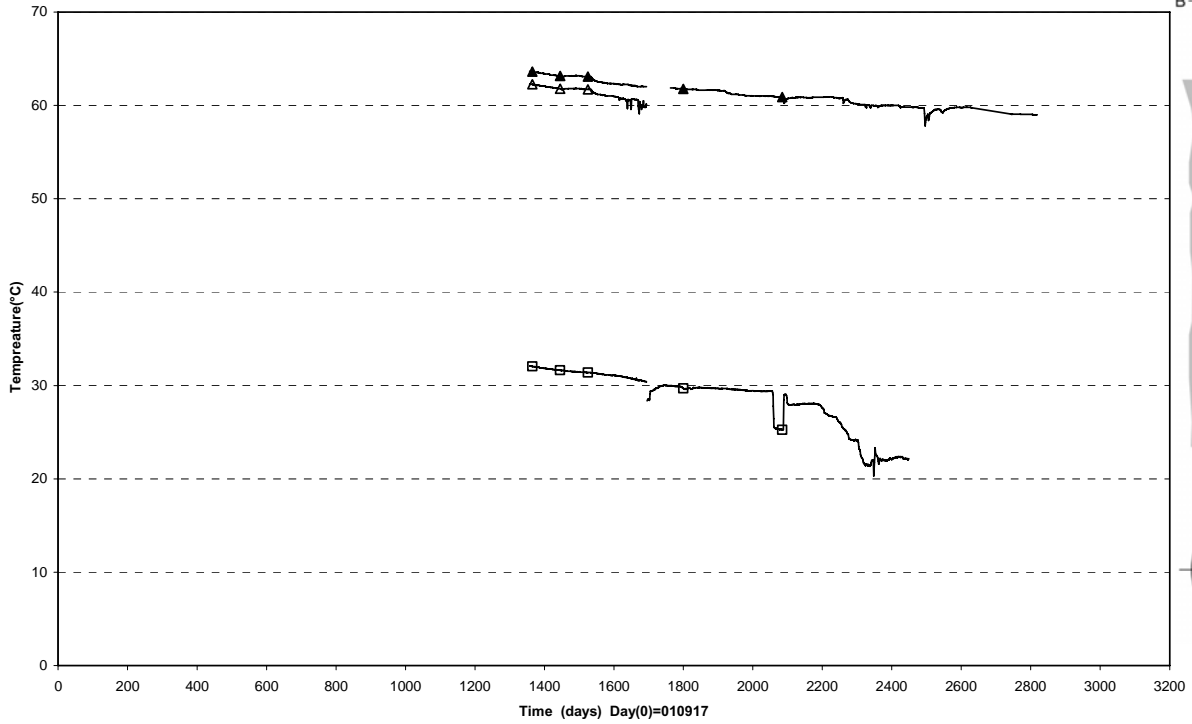
Prototype\Hole 1\ Cyl.1 (010917-091201) Temperature - Geokon
