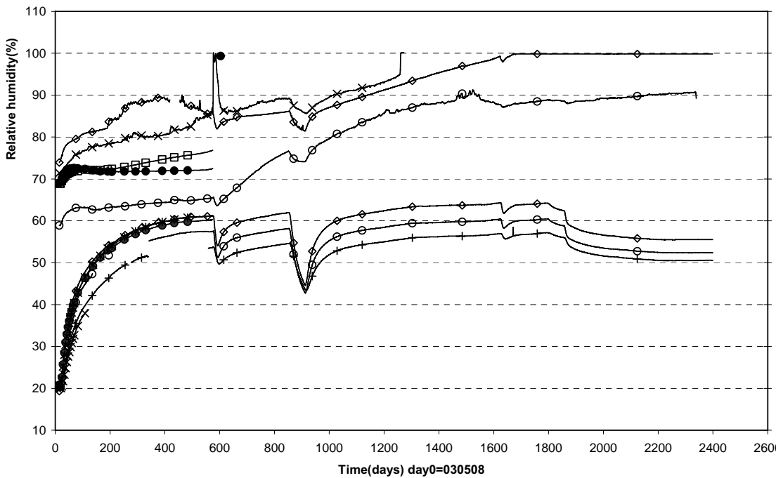
Prototype\Hole 6\Cyl.3 and Cyl.4 (030508-091201) Relative humidity
