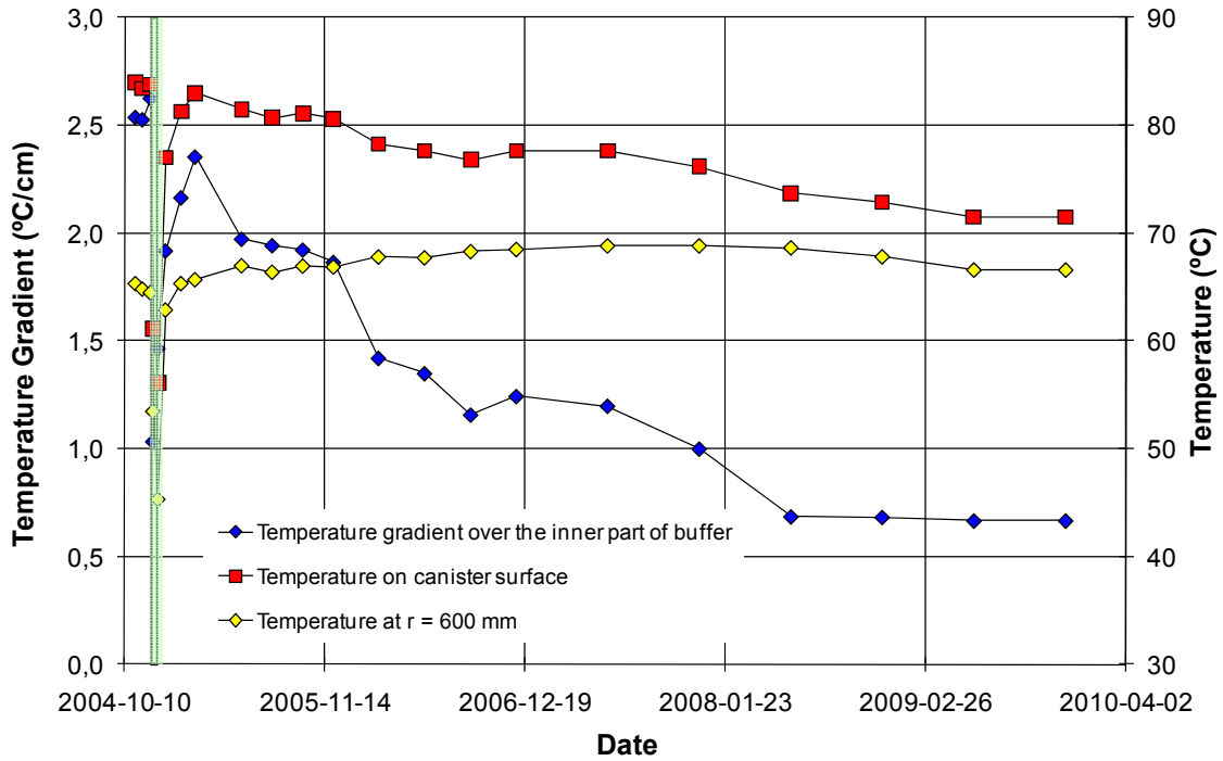
Figure 7-3. The temperature and temperature gradient over the inner part of the buffer plotted as function the date in deposition hole 5 block R5.
