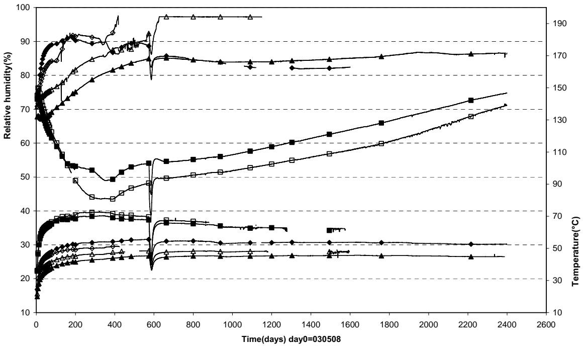
Prototype\Hole 5\Ring 10 (030508-091201) Relative humidity - Vaisala
