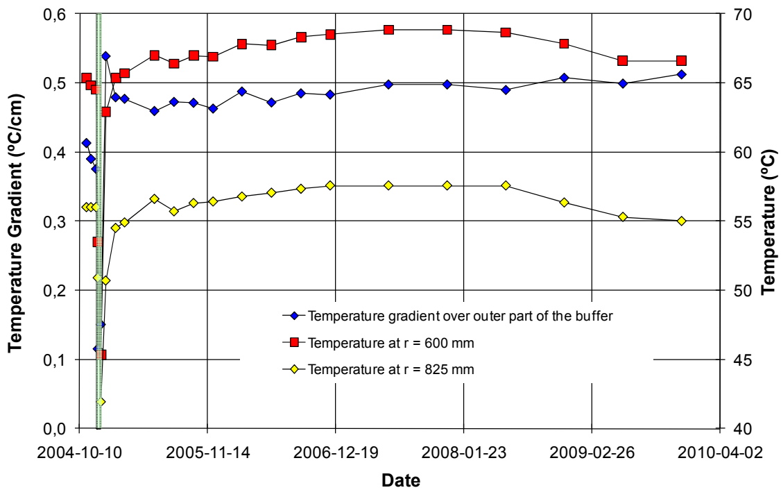
Figure 7-4. The temperature and temperature gradient over the outer part of the buffer plotted as function the date in deposition hole 5 block R5.
