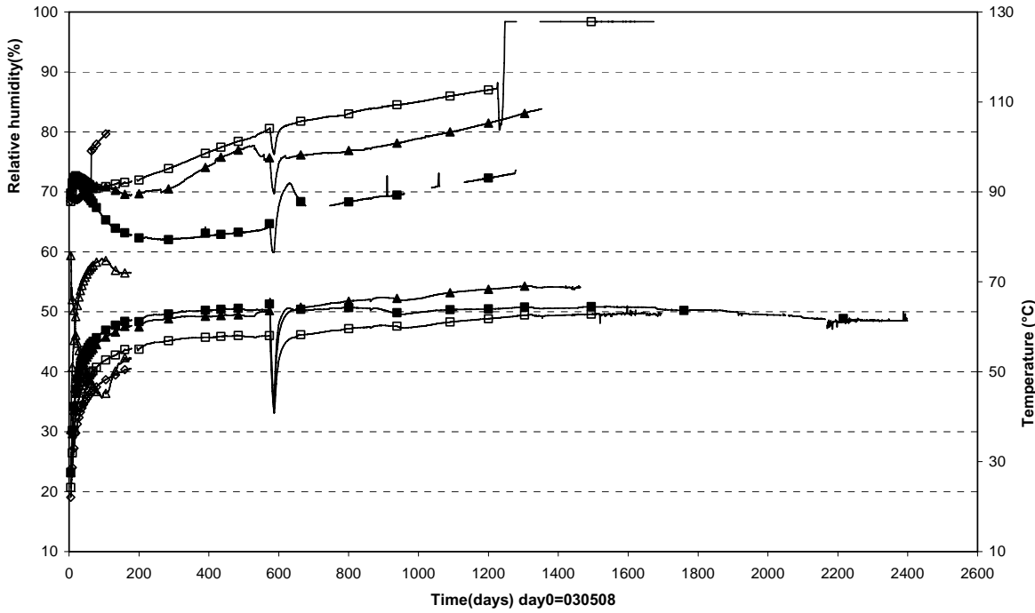
Prototype\Hole 5\Ring 5 (030508-091201) Relative humidity - Vaisala
