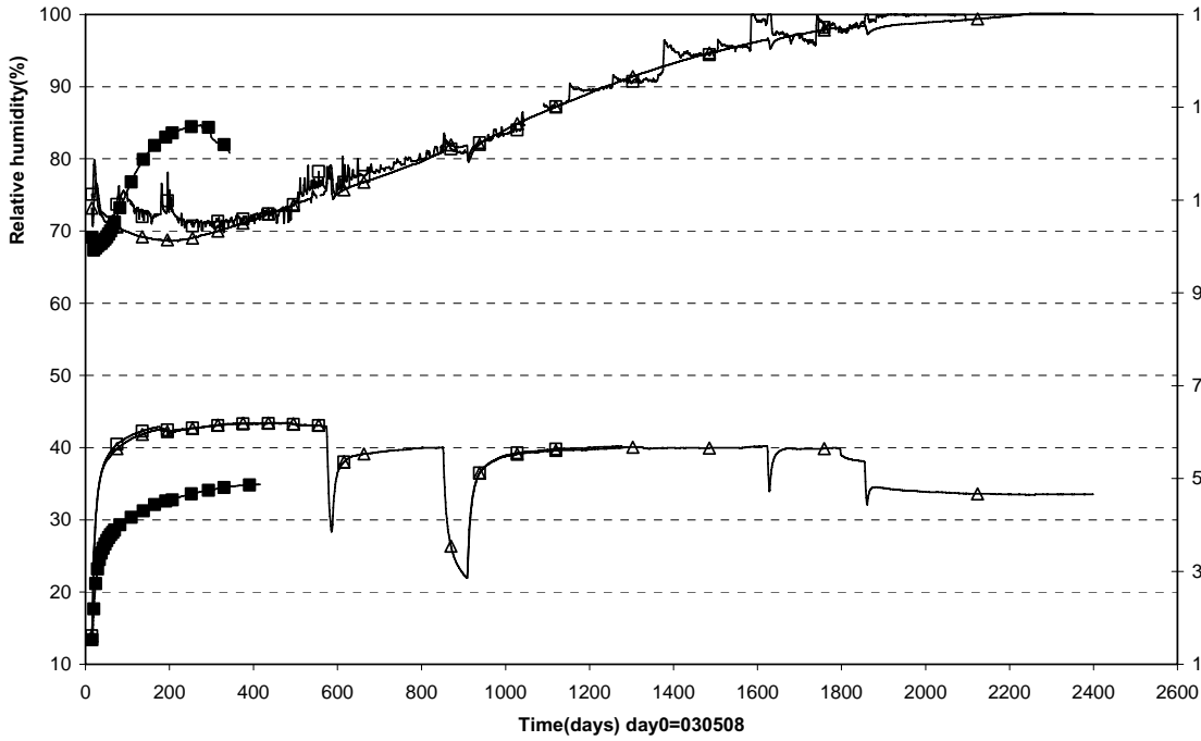
Prototype\Hole 6\Cyl.1 (030508-091201) Relative humidity
