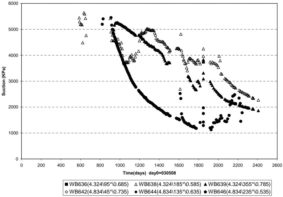
Prototypel Hole 6 \ Ring 8 and Ring 9 (030508-091201) Suction - Wescor
