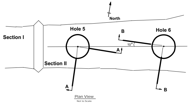
Figure 2.4 Plan views of complementary boreholes.
