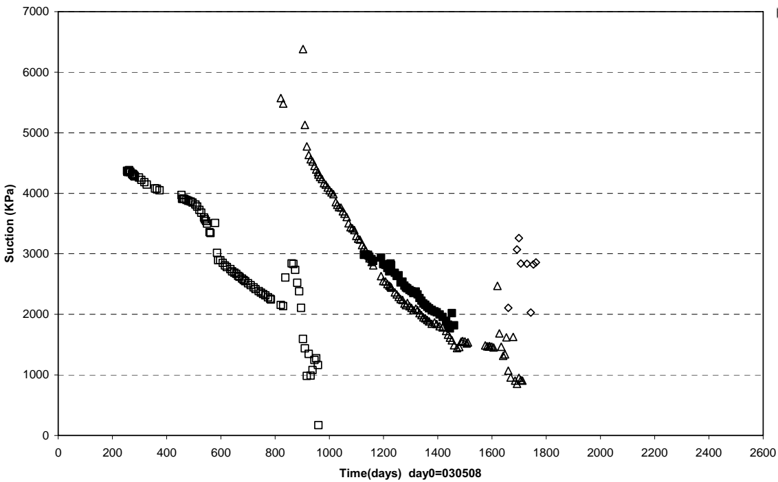
Prototypel Hole 6 \ Ring 1 and Ring 2 (030508-091201) Suction - Wescor
