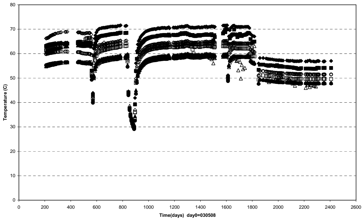
Prototypel Hole 6 \ Ring 5 and Ring 6 (030508-091201) Temperature - Wescor
