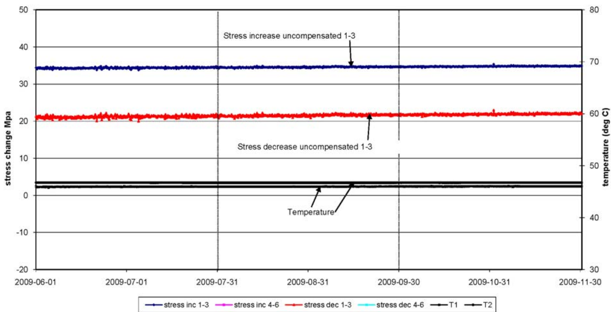
Biaxial stressmeter G5 Maximum stress increase and stress decrease in plane perpendicular to borehole axis
