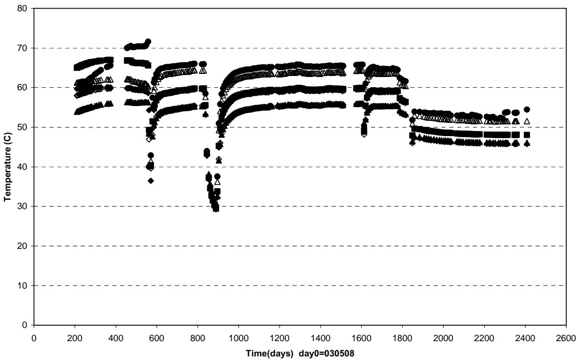
Prototypel Hole 6 \ Ring 8 and Ring 9 (030508-091201) Temperature - Wescor
