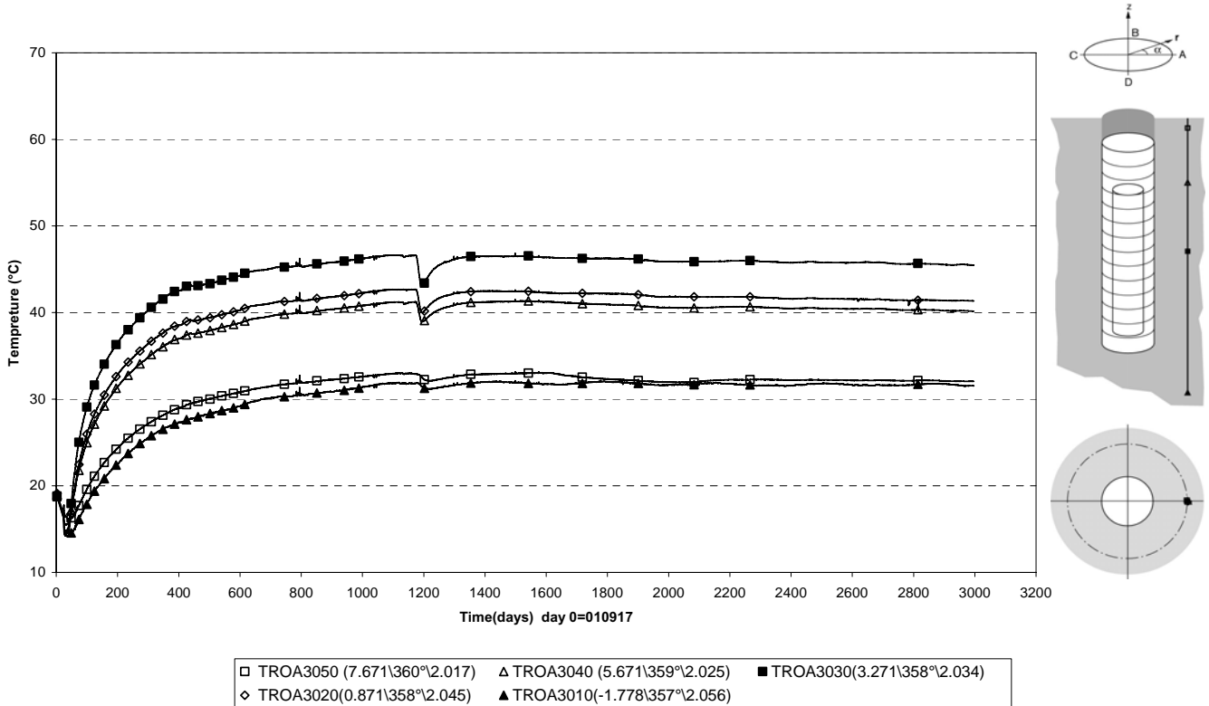
Prototype\Rock\Hole 4 (010917-091201) Temperature - Pentronic
