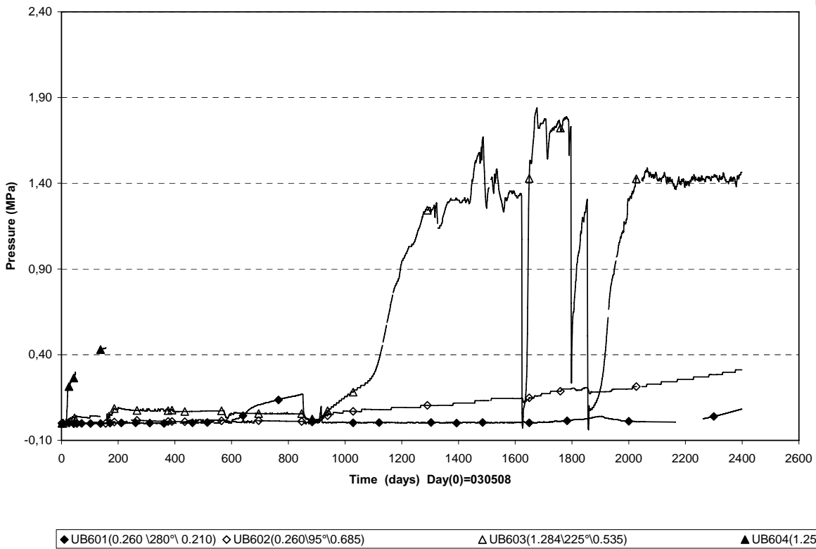
PrototypelHole6 \Cyl.1 and Ring2 (030508-091201) Pore pressure
