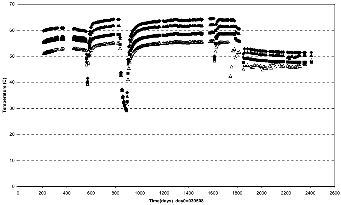
Prototypel Hole 6 \ Ring 6 and Ring 8 (030508-091201) Temperature - Wescor
