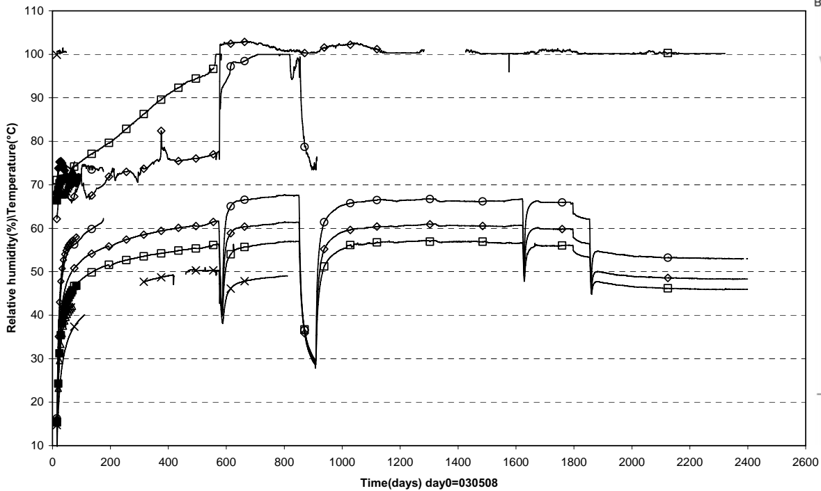
Prototype\Hole 6\ Ring 1 and Ring 2 (030508-091201) Relative humidity
