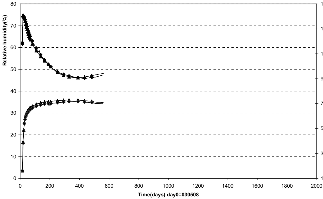
Prototype\Hole 6\ Ring10 (030508-091201) Relative humidity
