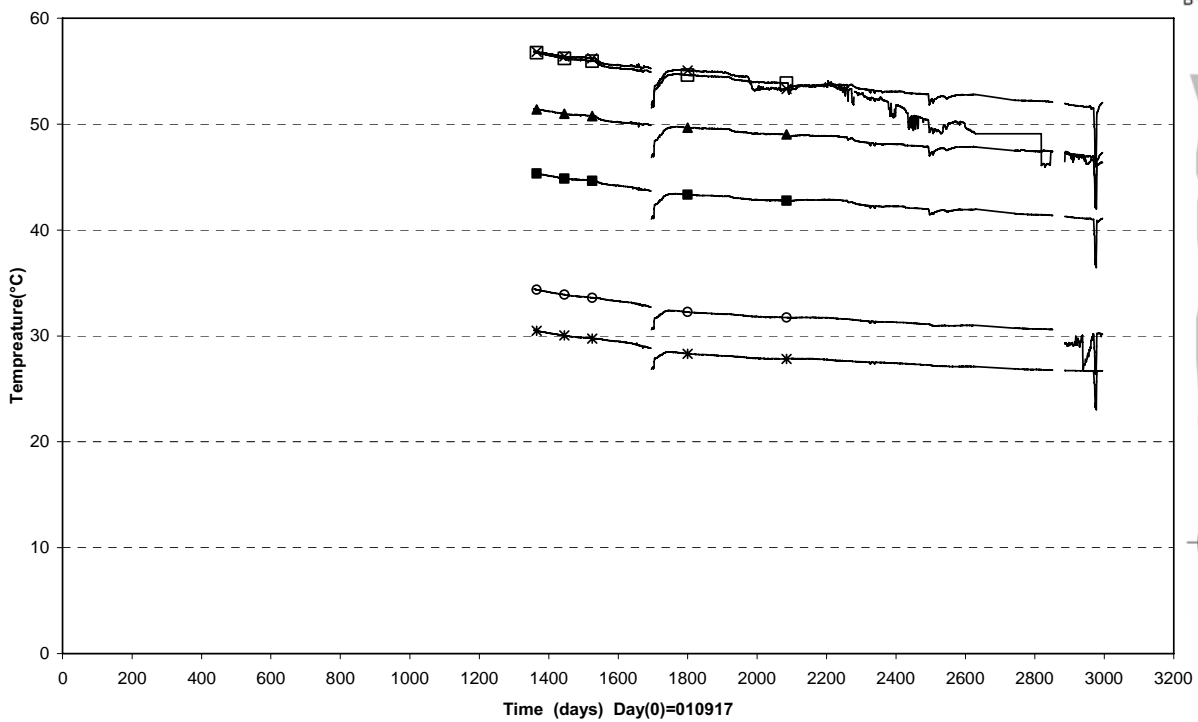
Prototype\Hole 1 (010917-091201) Temperature - Geokon
