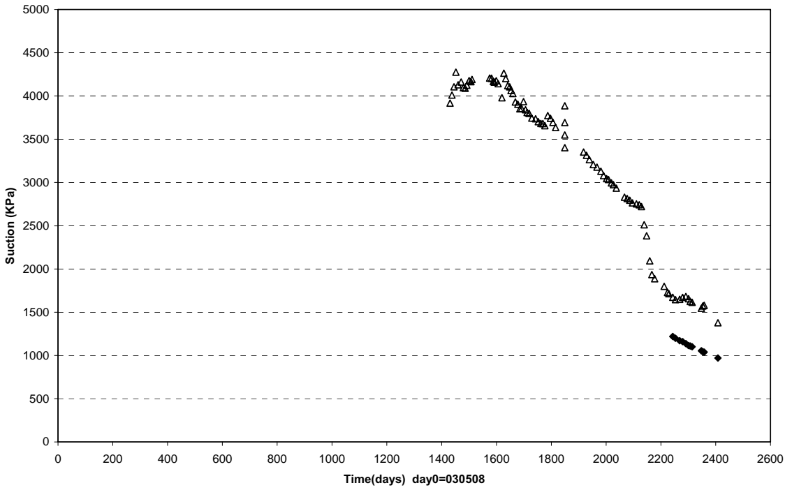
Prototypel Hole 6 \ Cyl1 (030508-091201) Suction - Wescor
