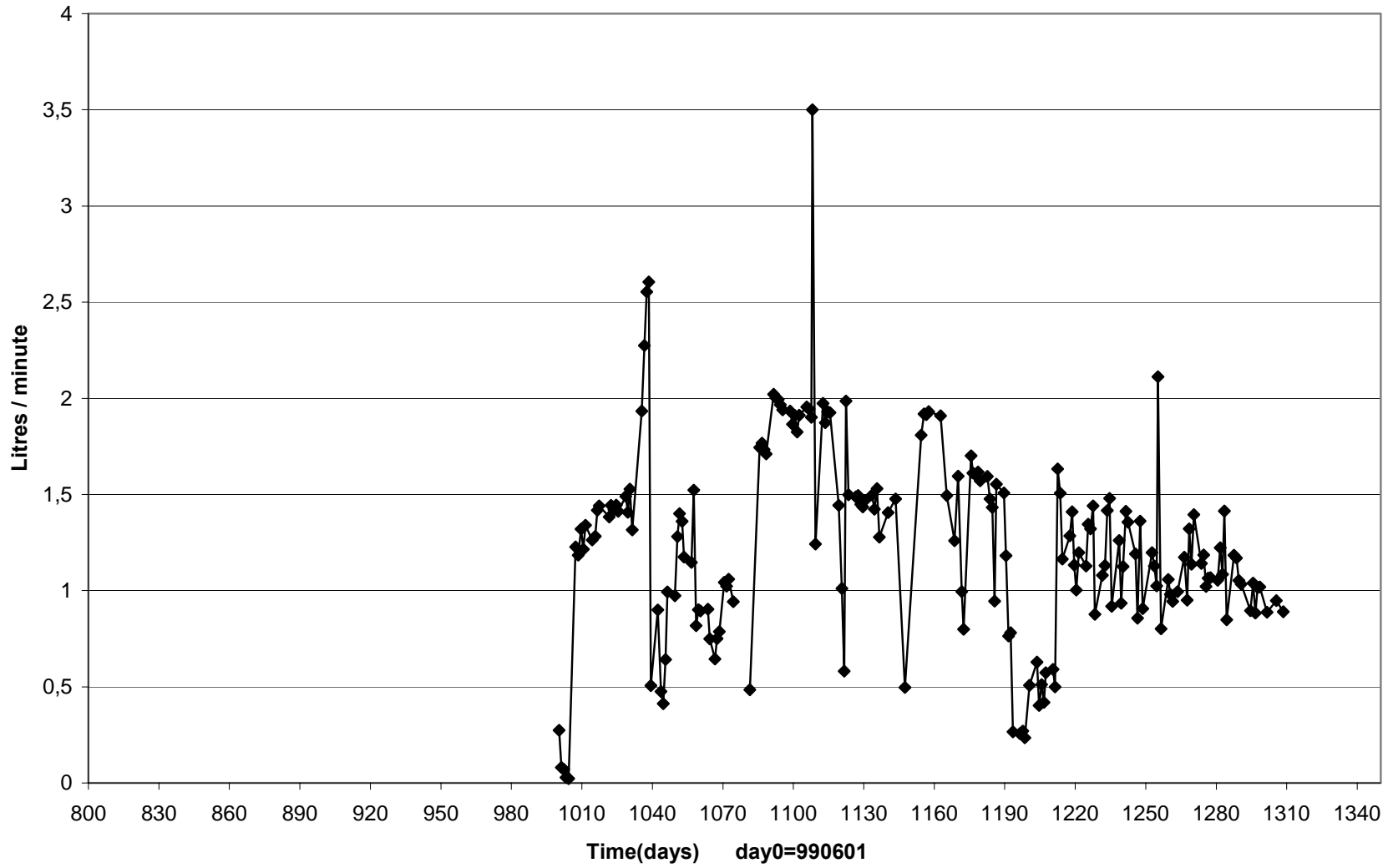
Water flow from inner part (010809-030101)
