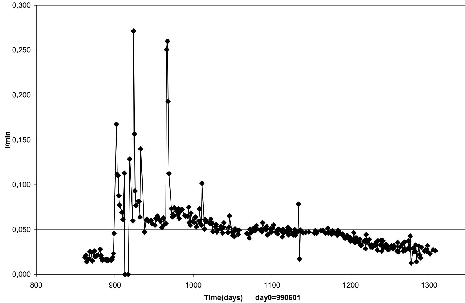
Water flow past plug (010809-030101)
