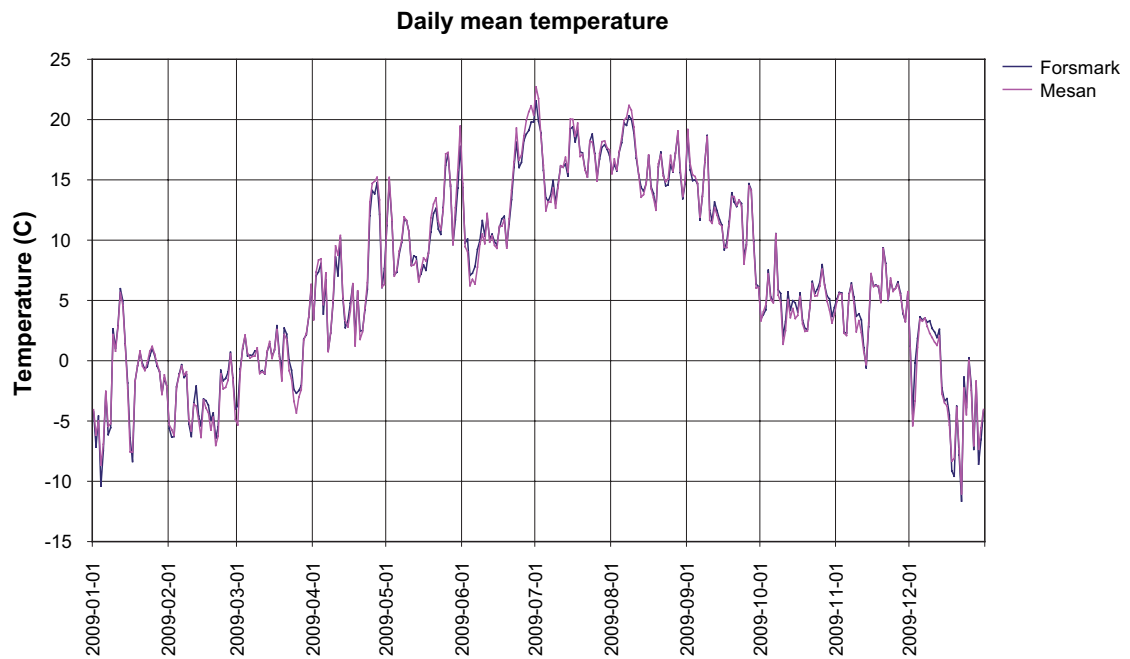
Figure A1-1. Temperature in °C, daily values, January 2009 – December 2009.
