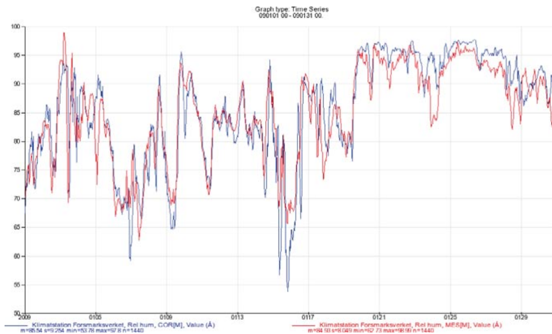
Figure A1-12. Relative humidity in %, 30-min. values, January 2009. (Blue line: measurements, red line: interpolated values from MESAN.)
