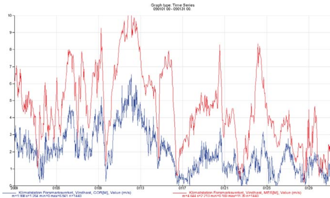
Figure A1-10. Wind speed in m/s, 30-min. values, January 2009. (Blue line: measurements, red line: interpolated values from MESAN.)
