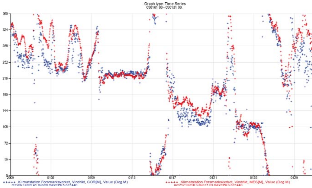
Figure A1-11. Wind direction in ^{\circ} , 30-min. values, January 2009. (Blue line: measurements, red line: interpolated values from MESAN.)
