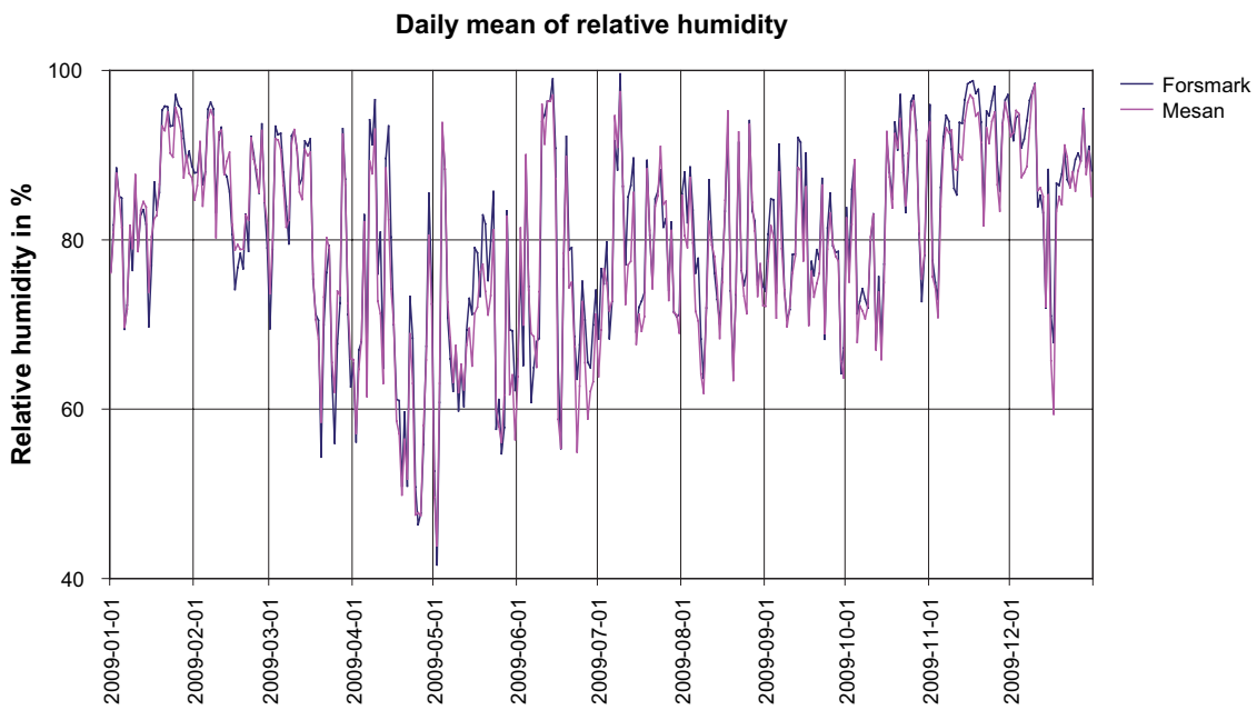
Figure A1-4. Relative humidity in %, daily values, January 2009 – December 2009.
