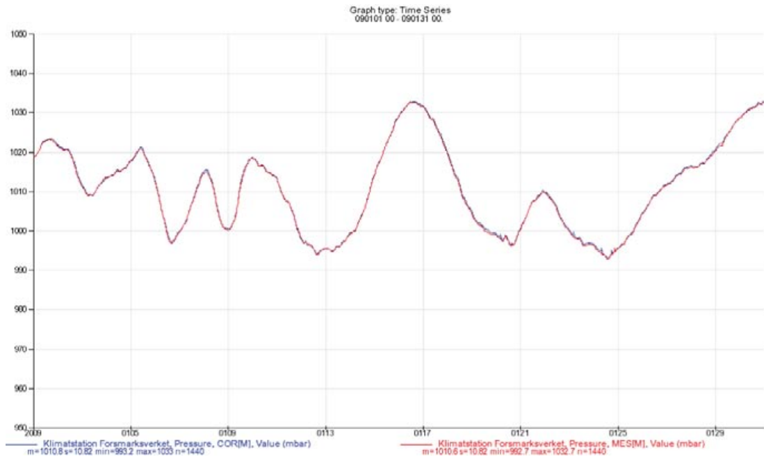
Figure A1-9. Barometric pressure in hPa, 30-min. values, January 2009. (Blue line: measurements, red line: interpolated values from MESAN.)
