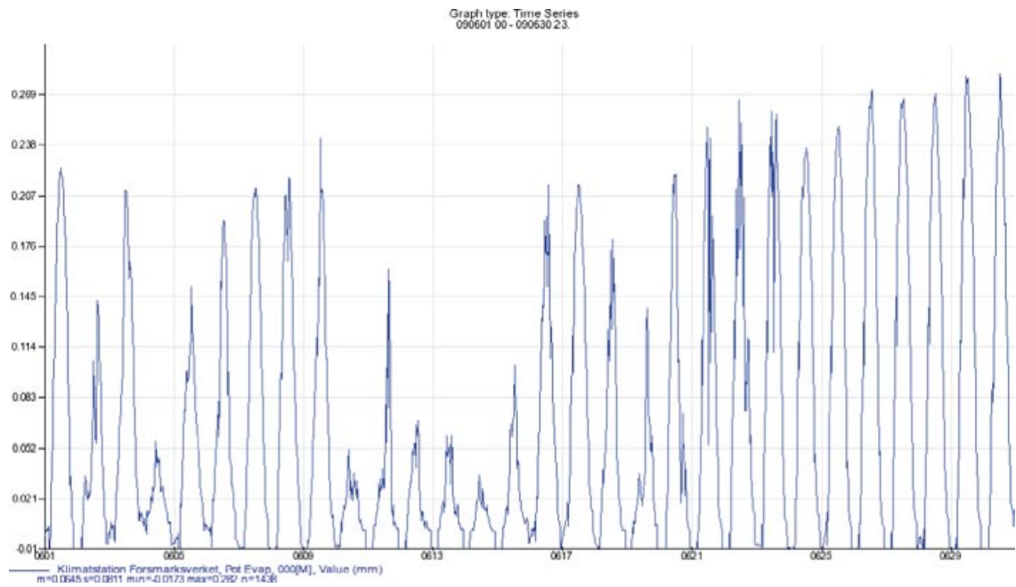
Figure A1-14. Potential evapotranspiration in mm, 30-min. values, June 2009.
