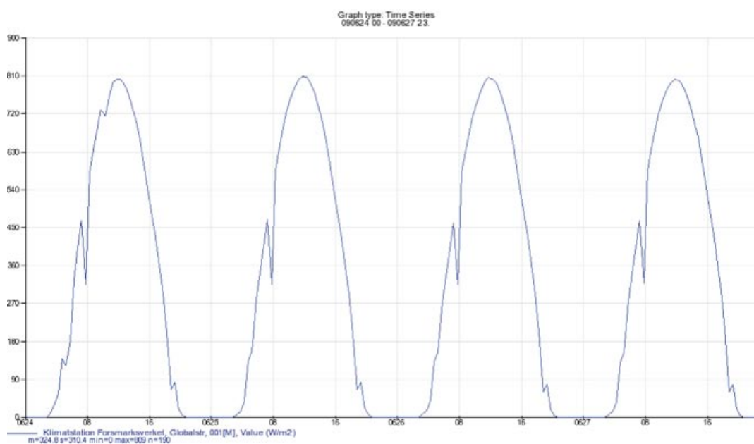
Figure 5-2. Global radiation 24–27 June 2009.
