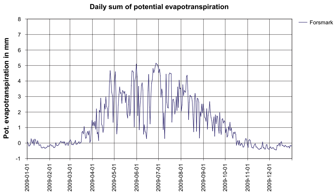
Figure A1-6. Potential evapotranspiration in mm, daily sum, January 2009 – December 2009.
