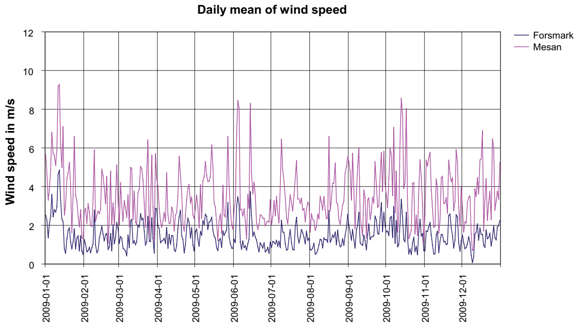
Figure A1-3. Wind speed in m/s, daily values, January 2009 – December 2009.
