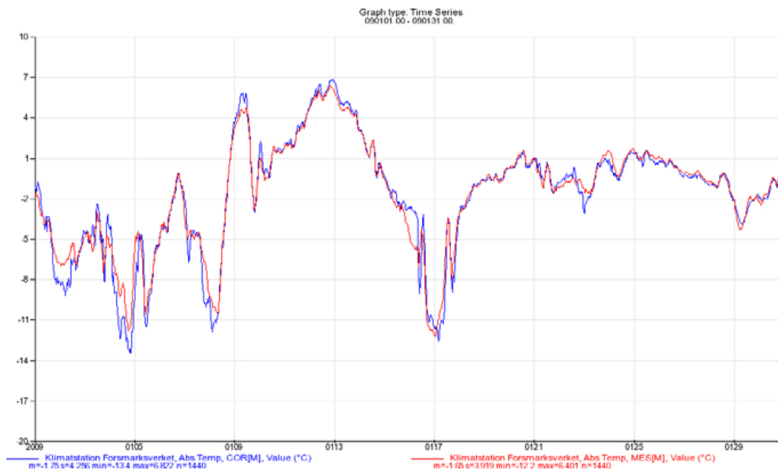
Figure A1-8. Temperature in °C, 30-min. values, January 2009. (Blue line: measurements, red line: interpolated values from MESAN.)
