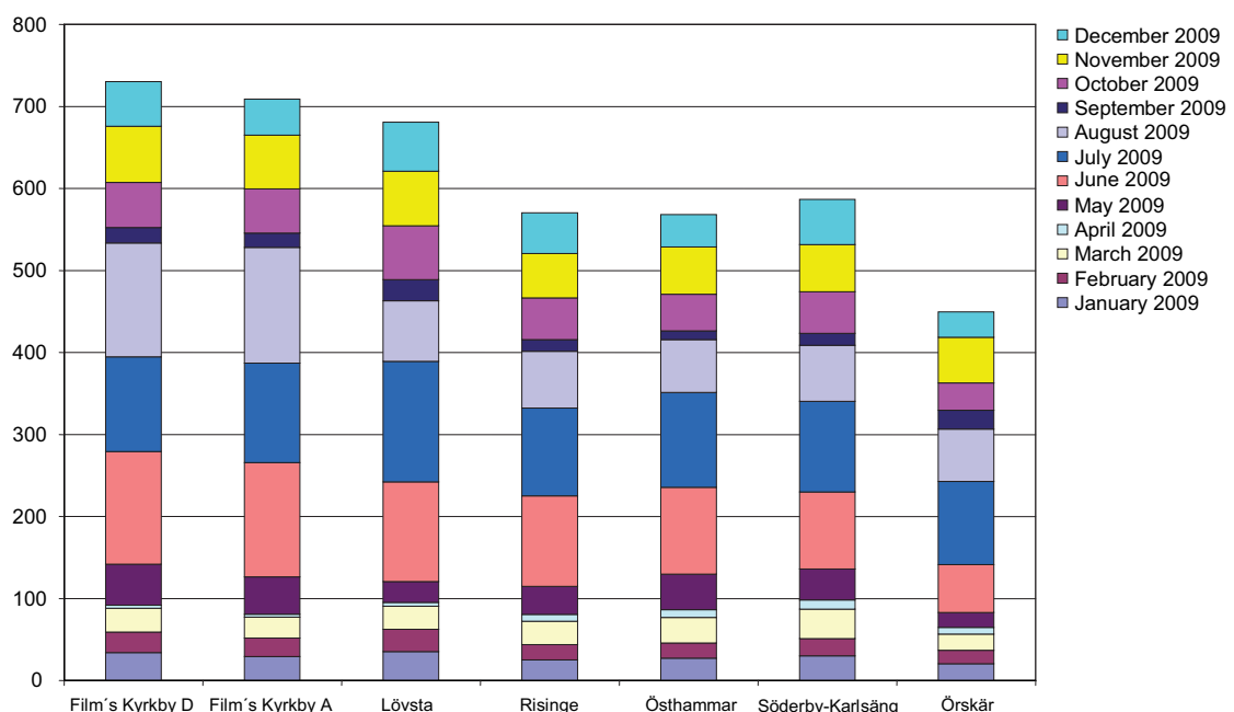
Figure 5-1. Monthly precipitation in mm at SMHI's stations. The values are not corrected for wind, wetting and evaporation losses.
