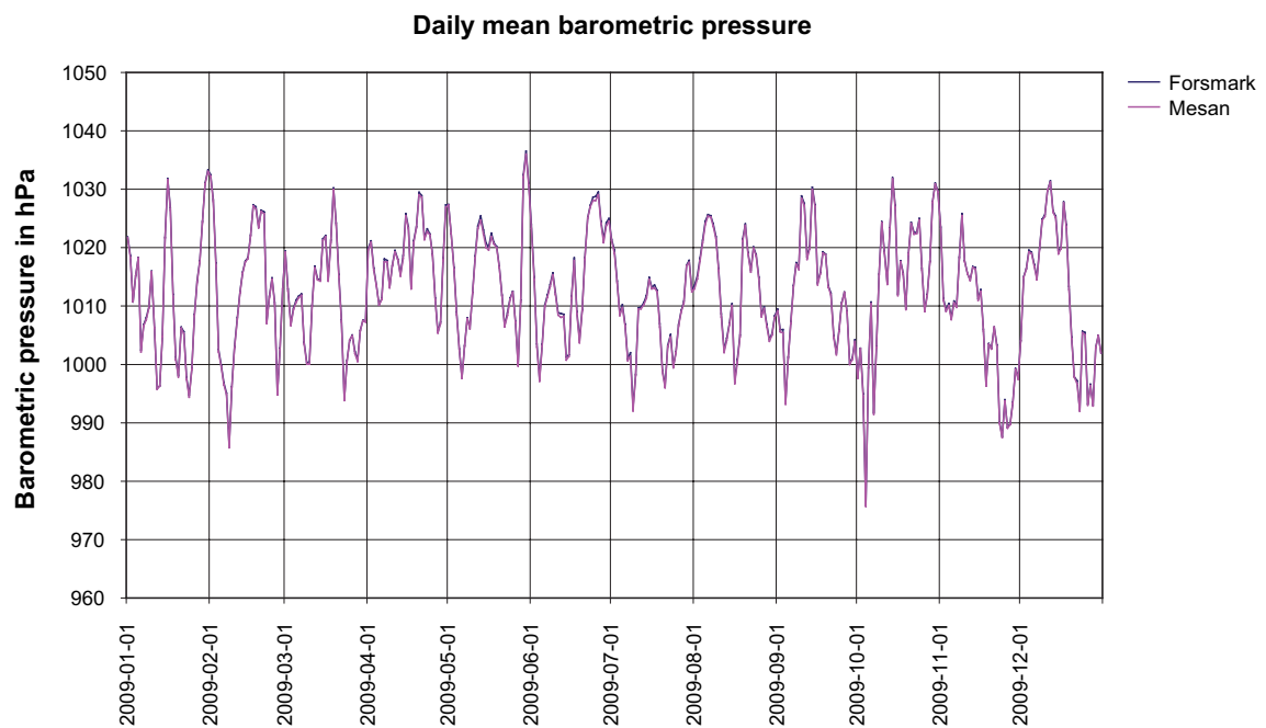
Figure A1-2. Barometric pressure in hPa, daily values, January 2009 – December 2009.
