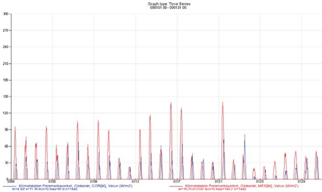
Figure A1-13. Global radiation in W/m^2 , 30-min. values, January 2009. (Blue line: measurements, red line: interpolated values from MESAN.)
