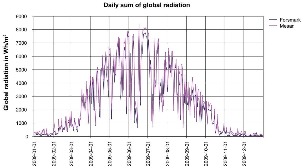
Figure A1-5. Global radiation in \text{Wh/m}^2 , daily sum, January 2009 – December 2009.
