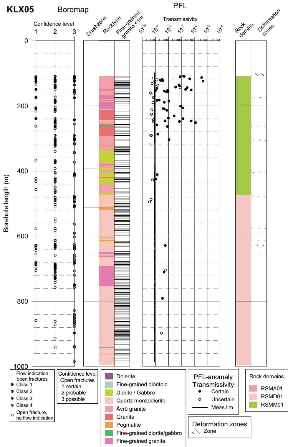
Figure 4-1. Correlations of hydraulic features based on PFL-f measurements, to mapped open/partially open fractures (all plotted as open fractures above) or crush zones in KLX05. Interpreted deformation zones and Rock Domains shown to the right. Fractures with PFL-anom confidence (flow indication class above) > 4 are not plotted.
