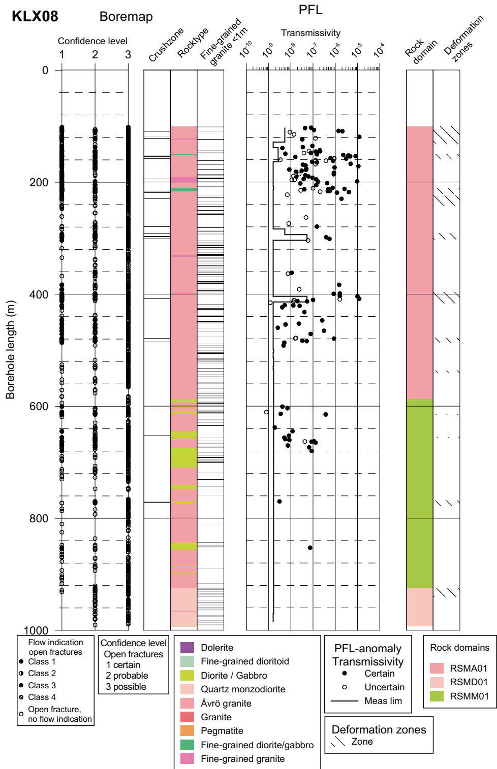
Figure 8-1. Correlations of hydraulic features based on PFL-f measurements, to mapped open/partly open fractures (all plotted as open fractures above) or crush zones in KLX08. Interpreted deformation zones and Rock Domains shown to the right. Fractures with PFL-anom confidence (flow indication class above) > 4 are not plotted.
