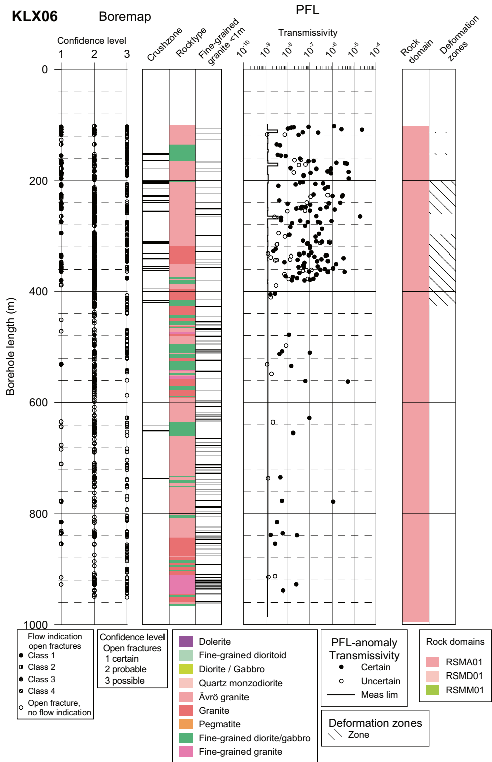
Figure 5-1. Correlations of hydraulic features based on PFL-f measurements, to mapped open/party open fractures (all plotted as open fractures above) or crush zones in KLX06. Interpreted deformation zones and Rock Domains shown to the right. Fractures with PFL-anom confidence (flow indication class above) > 4 are not plotted.
