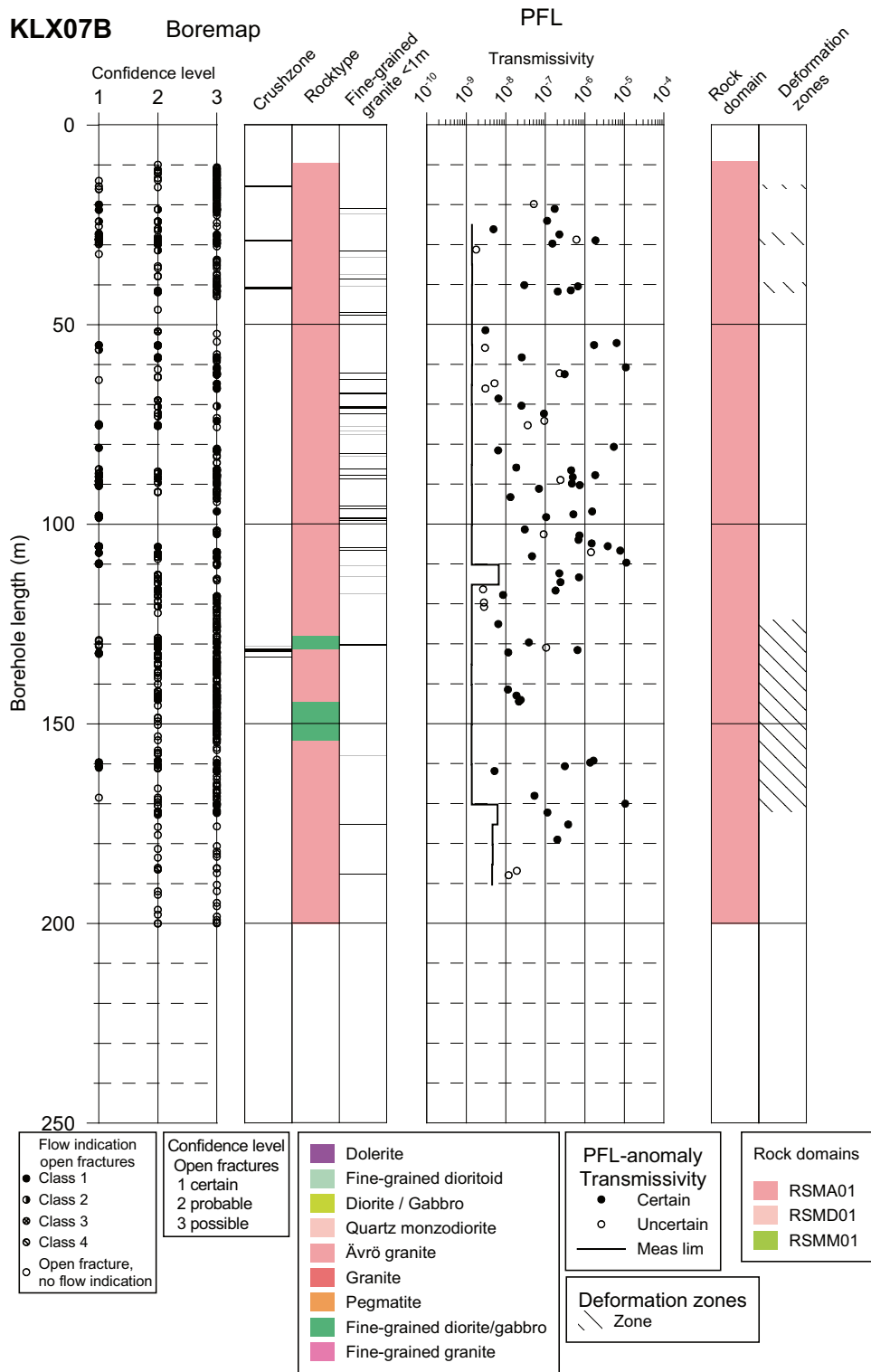
Figure 7-1. Correlations of hydraulic features based on PFL-f measurements, to mapped open/partly open fractures (all plotted as open fractures above) or crush zones in KLX07B. Interpreted deformation zones and Rock Domains shown to the right. Fractures with PFL-anom confidence (flow indication class above) > 4 are not plotted.
