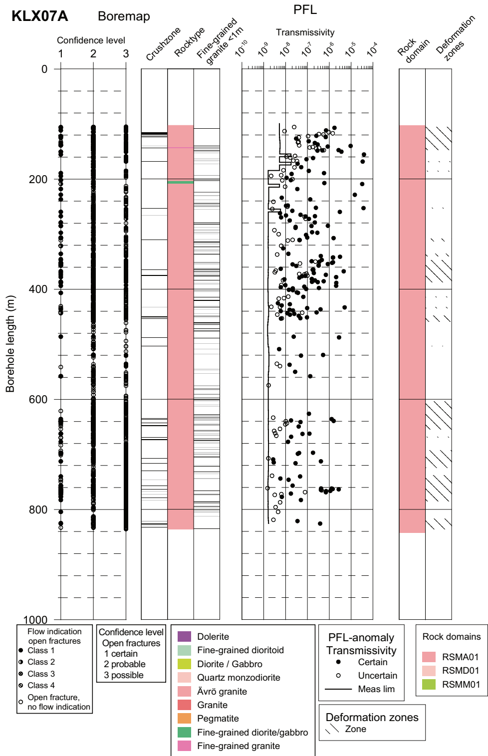
Figure 6-1. Correlations of hydraulic features based on PFL-f measurements, to mapped open/partially open fractures (all plotted as open fractures above) or crush zones in KLX07A. Interpreted deformation zones and Rock Domains shown to the right. Fractures with PFL-anom confidence (flow indication class above) > 4 are not plotted.
