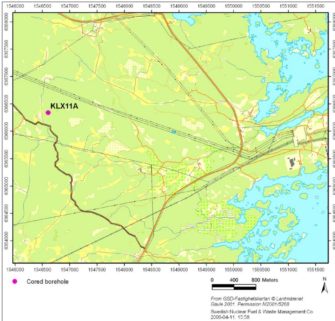
Figure 1-1. Site map showing the location of borehole KLX11A situated in the subarea of Laxemar.
