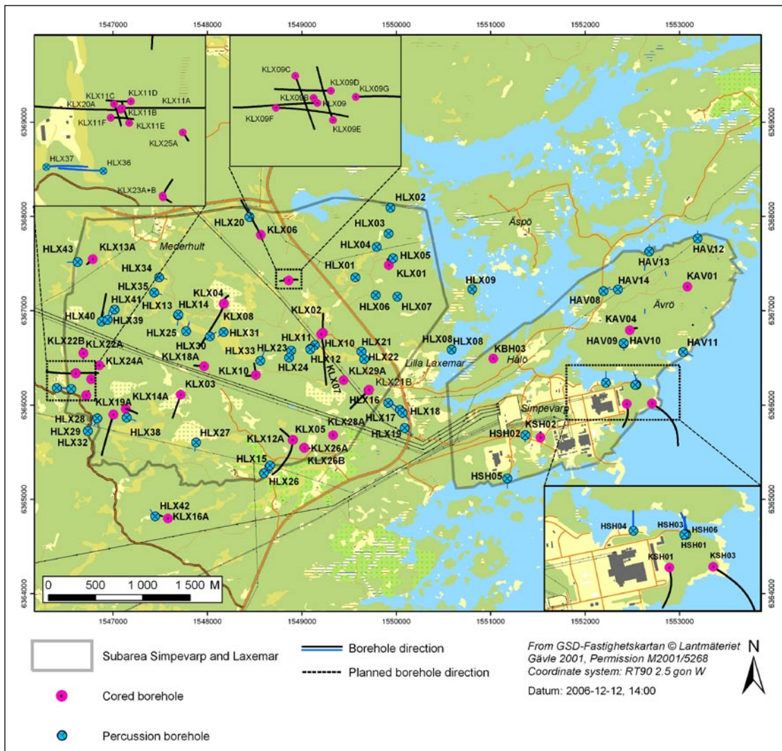
Figure 1-1. Location of all telescopic boreholes drilled up to December 2006. The projection of each borehole on the horizontal plane at top of casing is also shown in the figure.
