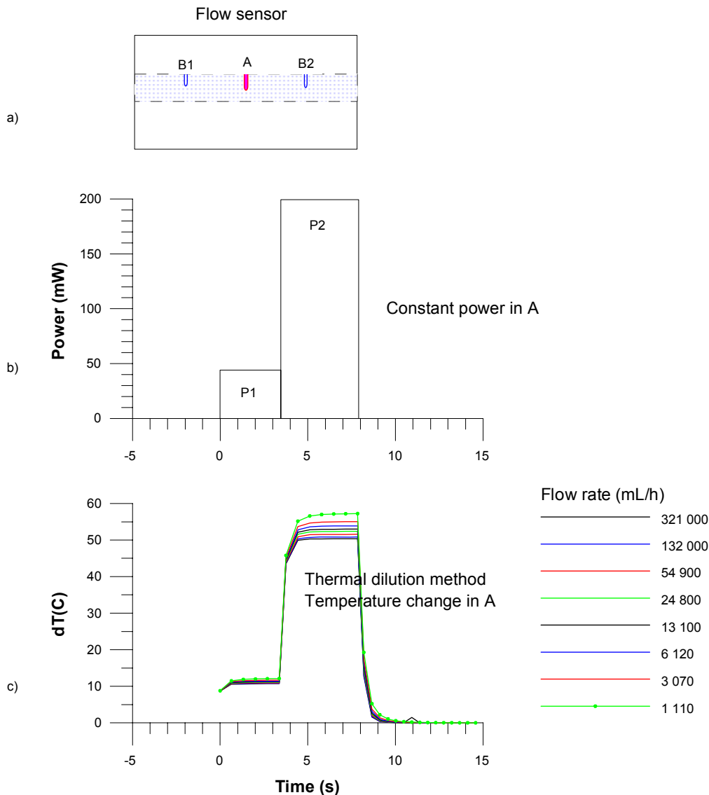
Figure 3-4. Flow measurement, flow rate > 600 mL/h.
