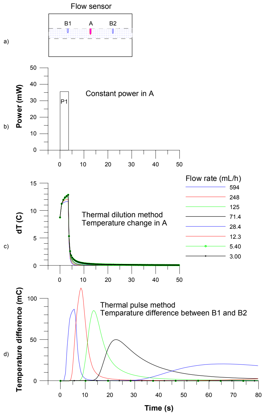
Figure 3-3. Flow measurement, flow rate <math>< 600 \text{ mL/h}</math>.
