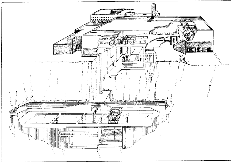
Figure 4-3. The Swedish interim storage facility for spent nuclear fuel, CLAB.
