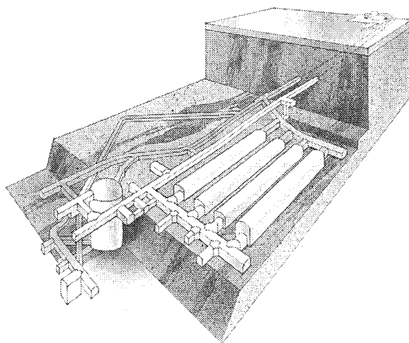
Figure 4-2. The SFR repository in Forsmark.
