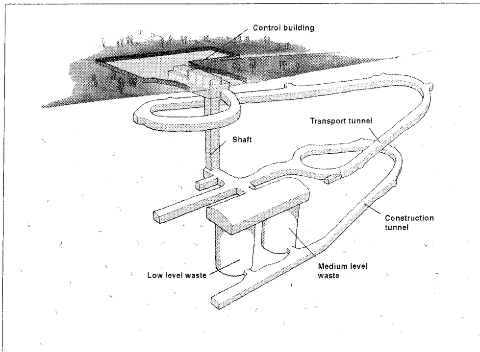
Figure 4-4. The Finnish final repository for low- and medium level radioactive waste, VLJ repository.
