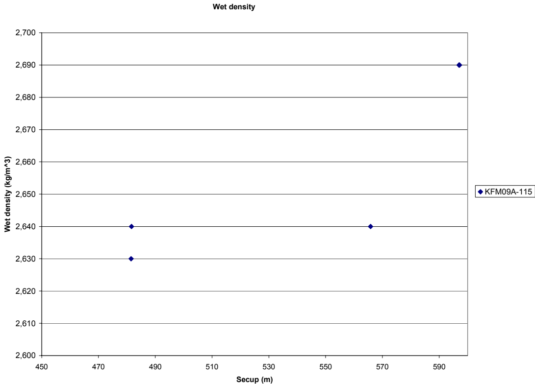
Figure 5-1. Density versus sampling level (borehole length).
