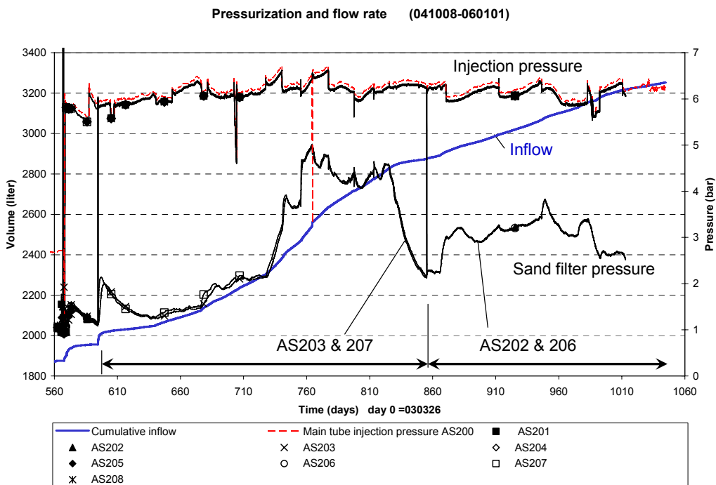
Figure 5-2. Pressurization and flow rate after the second hydraulic test mid-October 2004. AS200 is the main tube. AS201 – AS 208 is individual injection tubes. The actual water pressure in the sand filter was only measured at two points.
