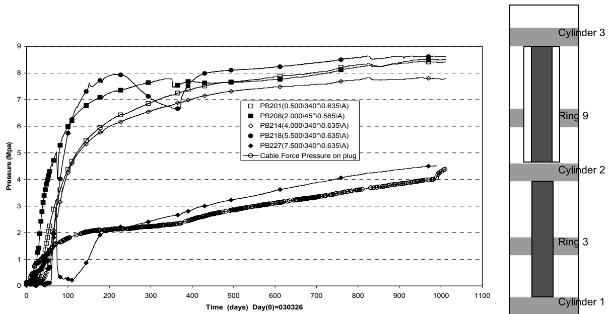
Figure 5-10. Axial pressure measured in different sections.
