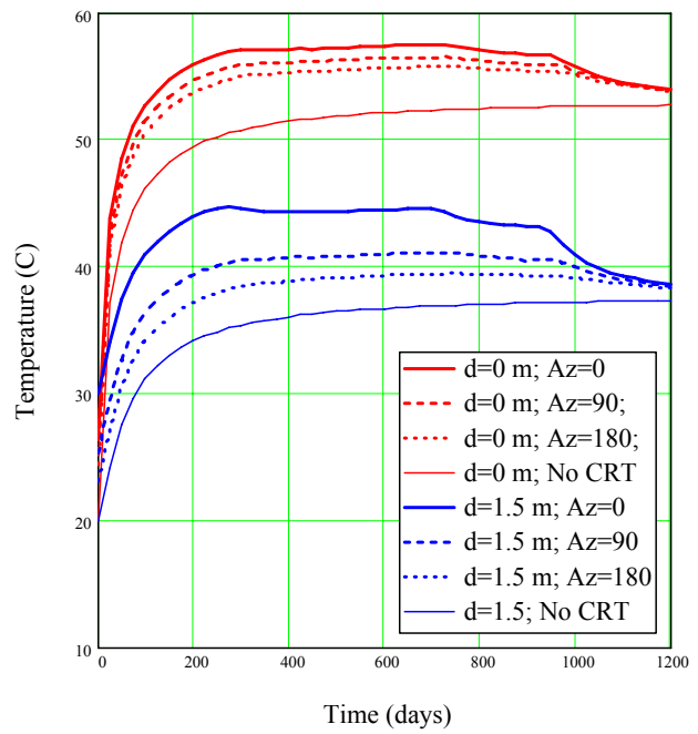
Figure 5-4. Analytical model of thermal influence of CRT on TBT. Upper: CRT heat load. Lower left: Geometry of model. Lower right: calculated temperatures.
