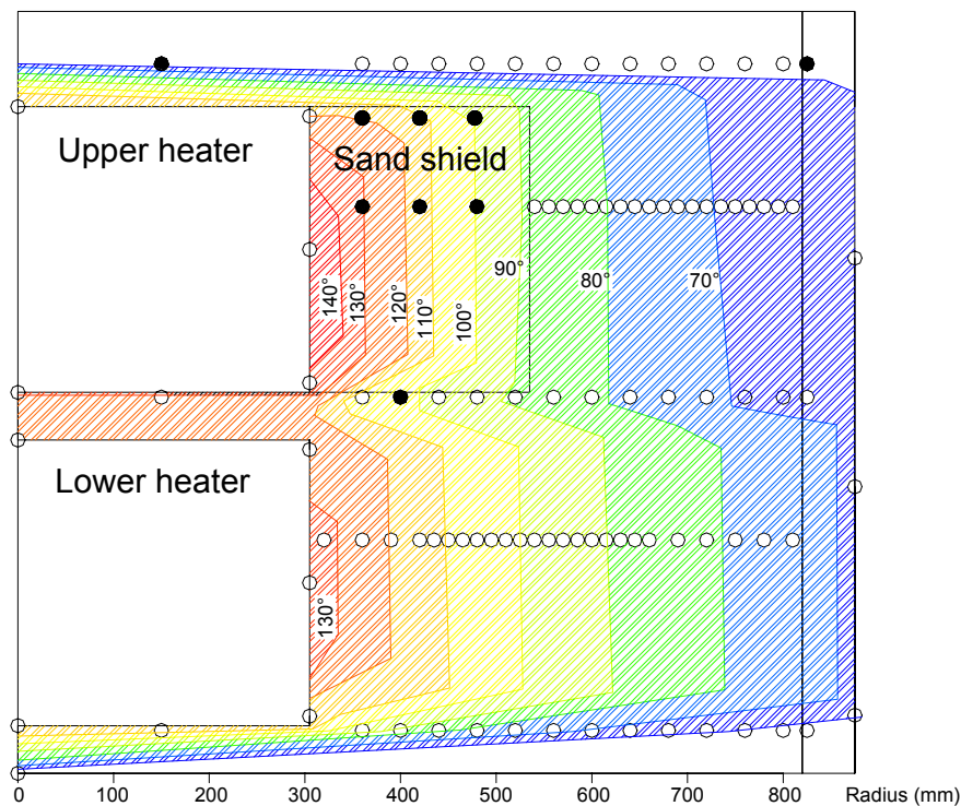
Figure 5-3. Temperature distribution at January 1, 2006. Rings indicate sensor positions. Filled rings indicate sensors out of order.
