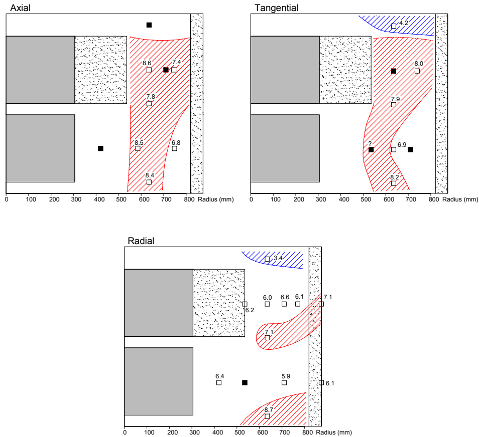
Figure 5-9. Total pressure distribution at January 1, 2006. Values in MPa. Boxes are sensor positions. Filled boxes indicate sensors out of order. Levels above 7 MPa marked red; below 5 MPa marked blue.
