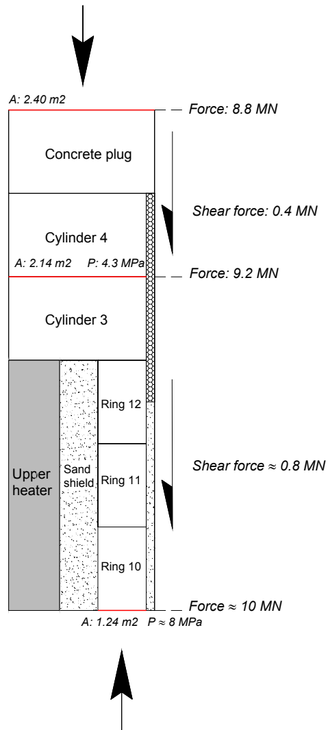
Figure 5-11. Schematic of vertical forces acting on the upper part of the package (data from 2005-07-01).
