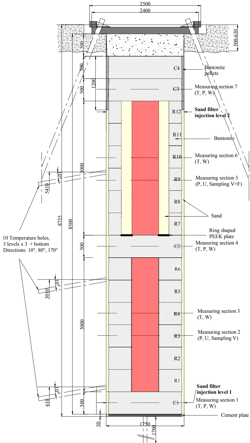
Figure I-1. Schematic view showing the layout of the experiment and the numbering of bentonite blocks. The lower heater is denominated No. 1 and the upper heater is No. 2.
