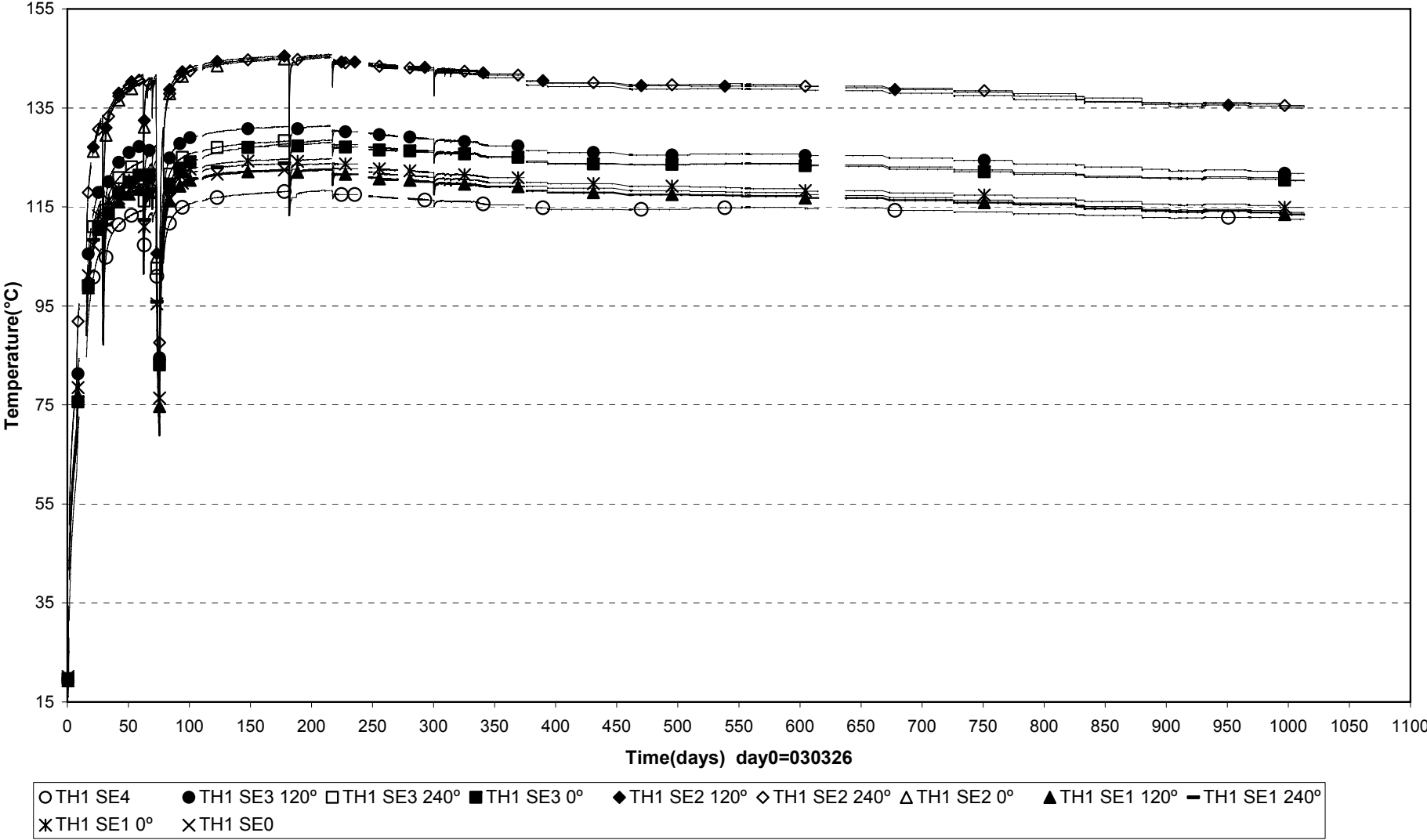
External temperatures Heater 1 (030326-060101)
