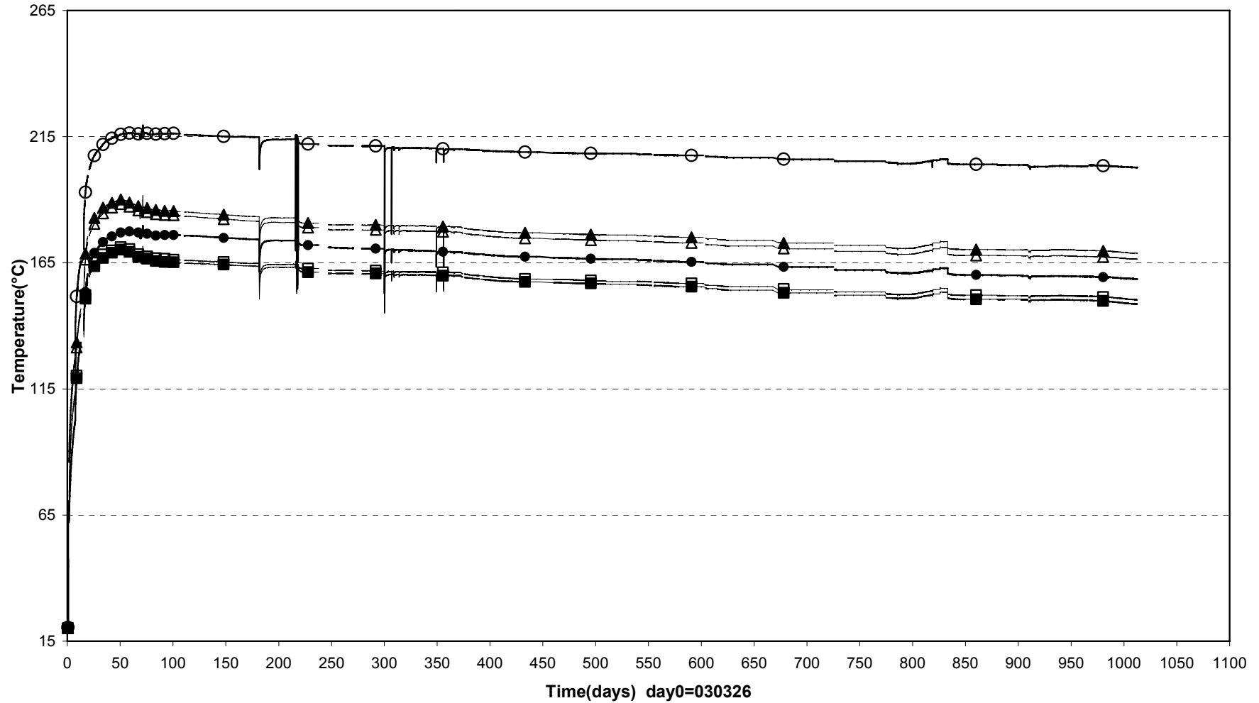
Internal temperatures Heater 2 (030326-060101)
