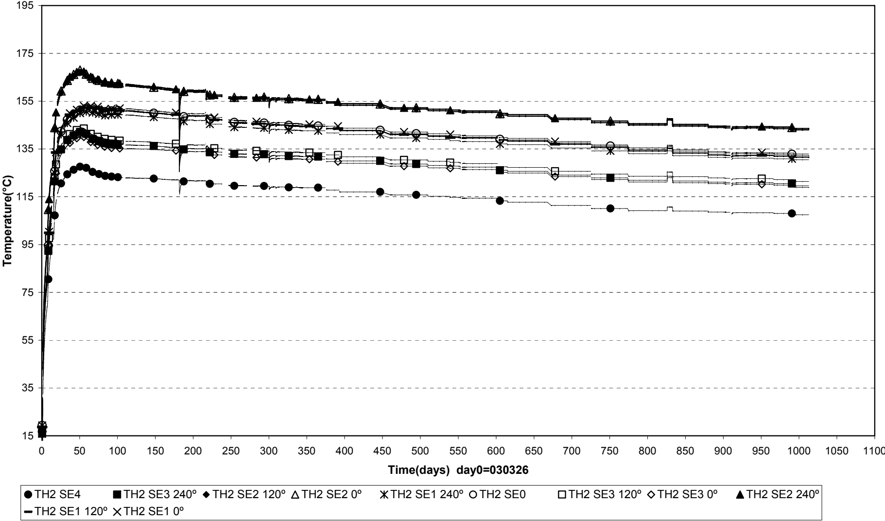
External temperatures Heater 2 (030326-060101)
