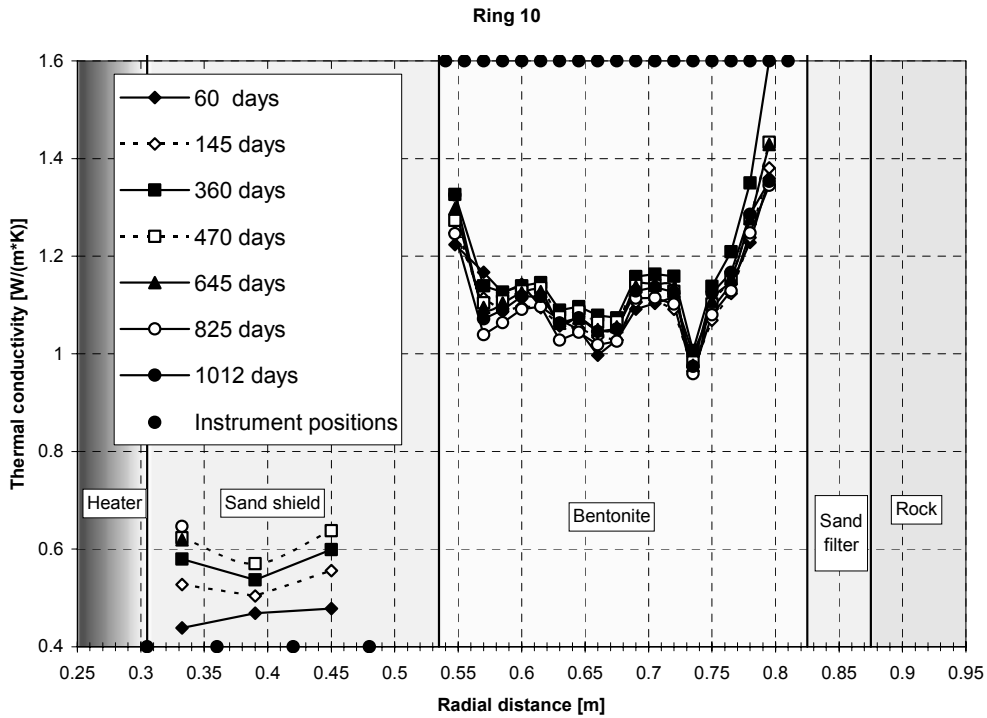
Figure 5-6. Thermal conductivity as computed from slopes of distance-temperature relation.
