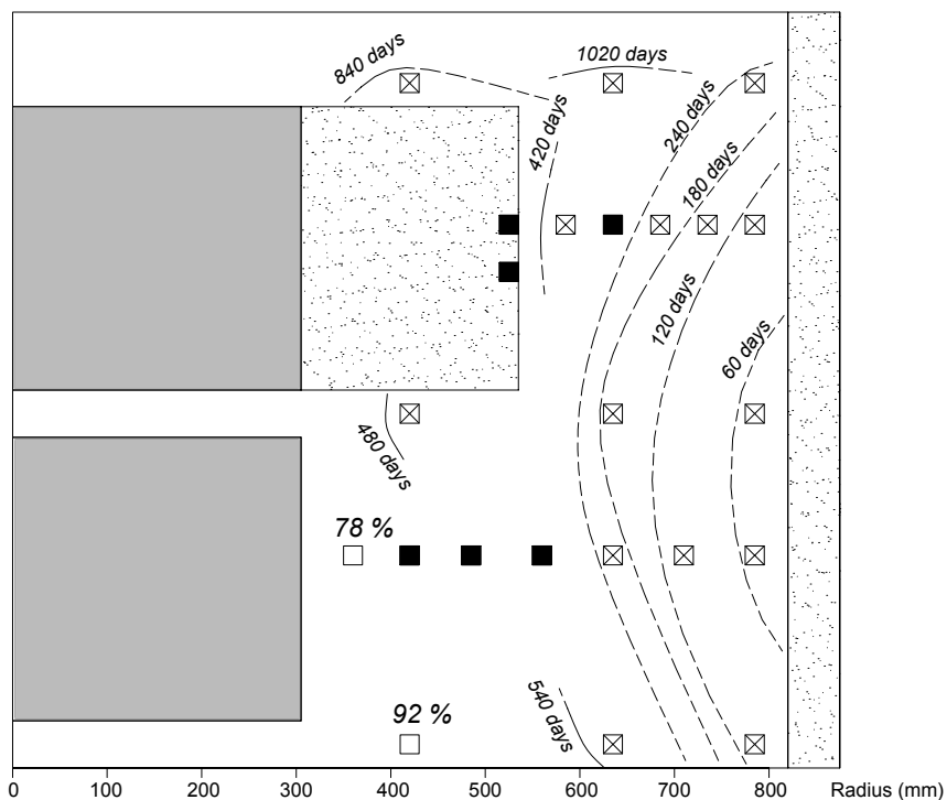
Figure 5-8. Occurrences of saturation up till January 1, 2006. Boxes are sensor positions. Ticked boxes indicate saturation. Filled boxes indicate sensors out of order. Percentages are current RH values.
