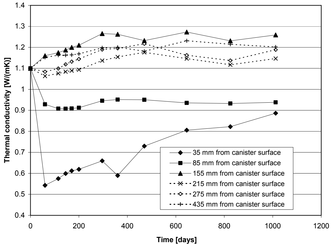
Figure 5-7. Thermal conductivity development in ring 4.
