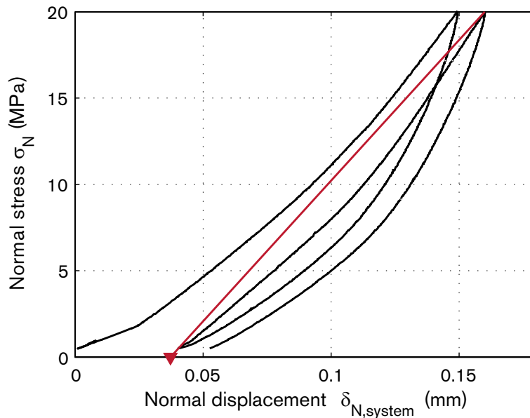
Figure 4-3. Results from a normal loading test with a steel specimen cast in epoxy. The black curve is showing the results from the tests where the steel deformation has been subtracted from the results. The red line, which is representing the secant of the loading curve during the second load cycle, is intersecting the points at full unloading and full loading. The extension of the line is intersecting the zero stress level at the displacement \delta_{N,0} . This point is regarded as a theoretical starting point of the second load cycle and is marked with a filled triangle in the figure.
