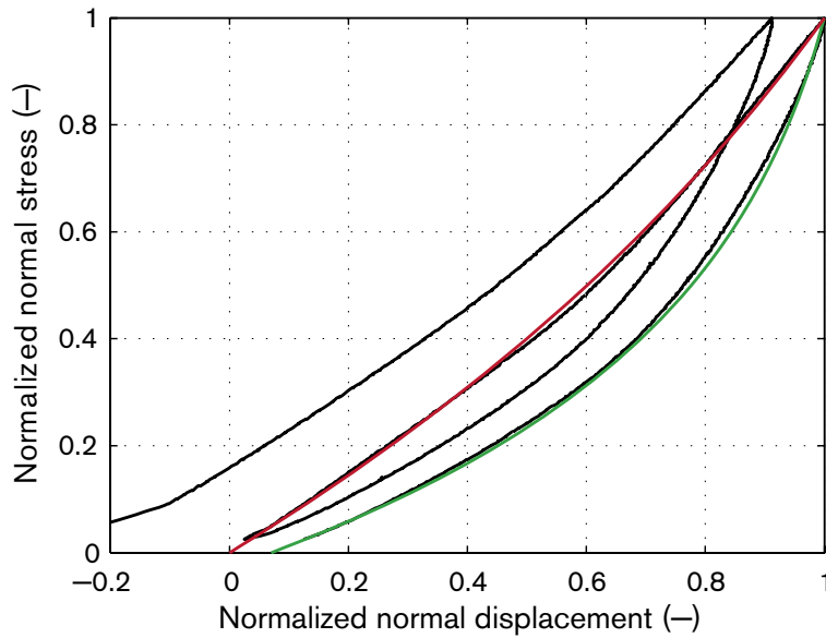
Figure 4-4. Results from normal loading test on a steel specimen with normalized result parameters. The black curve is showing the results from the tests where the steel deformation has been subtracted from the results. The red and the green curves are showing the fitted approximating functions for the loading and unloading responses during the second load cycle.
