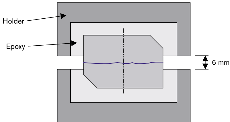
Figure 4-2. Specimen cast in the specimen holder.
