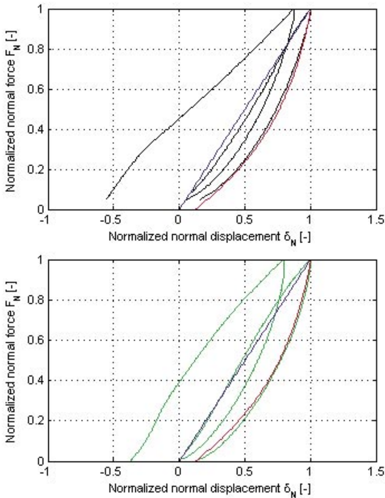
Figure 4-2. Results from normal loading tests on a steel specimen. The upper diagram is showing the normalized results from the 28 kN normal load cycle (black) and the lower diagram displays the normalized results from the 110 kN normal load cycle (green). The blue curve is the linear approximation for loading of the second load cycle and the red curve is the non-linear approximation for unloading of the second load cycle.
